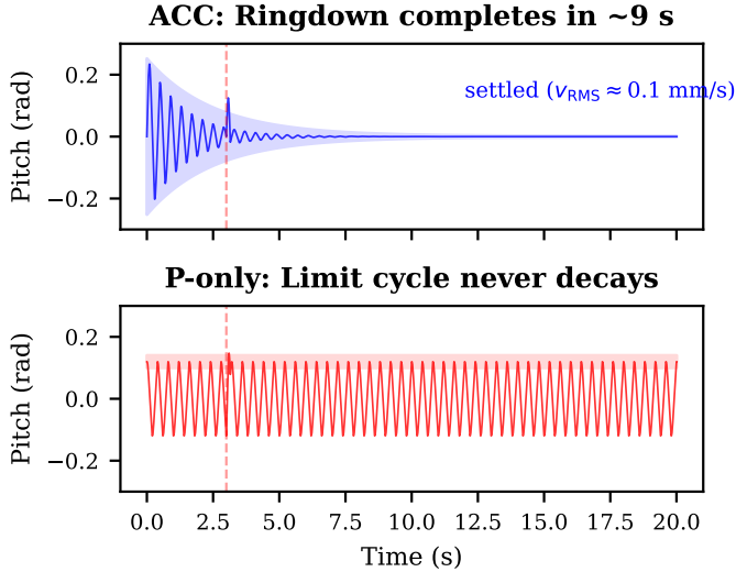
Fig. 4. Post-push pitch ringdown: ACC (top) vs. P-only (bottom). 90 N push applied at t = 3 s. ACC ringdown completes in \sim 9 s; P-only oscillation persists indefinitely due to equilibrium bias.
