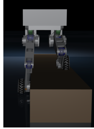
Fig. 6. One-wheel curb (20 cm). With the per-leg height split: 14.9 \pm 0.1 ^\circ straddle roll, 10/10 settled. With a symmetric posture (split removed): the curb-side leg cannot fold far enough, roll diverges past 60^\circ within 0.8 s of curb entry, 0/10.
