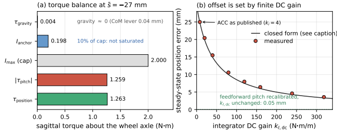
Fig. 7. Static torque balance of the sagittal parking offset. (a) Measured sagittal torques at the \bar{s} = -27 mm parking point. The gravity moment about the wheel axle is 0.0040 Nm and the anchor integral sits at 10% of its clamp, so the offset is neither gravity-driven nor a saturation artifact; the balance is between the pitch and position loops. (b) Steady-state position error against integrator DC gain k_{I,dc} of Eq. (26), swept over k_i \in [4, 160] at fixed leak. The curve is Eq. (27) evaluated with the baseline \tau_{pitch} ; using each run's own measured \tau_{pitch} the closed form tracks all twelve gain and height points to within 0.92%. The dotted line is the same controller with the feedforward pitch reference recalibrated and k_{I,dc} left unchanged.
