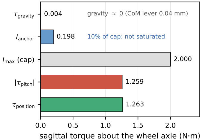
(a) torque balance at \bar{s} = -27 mm
