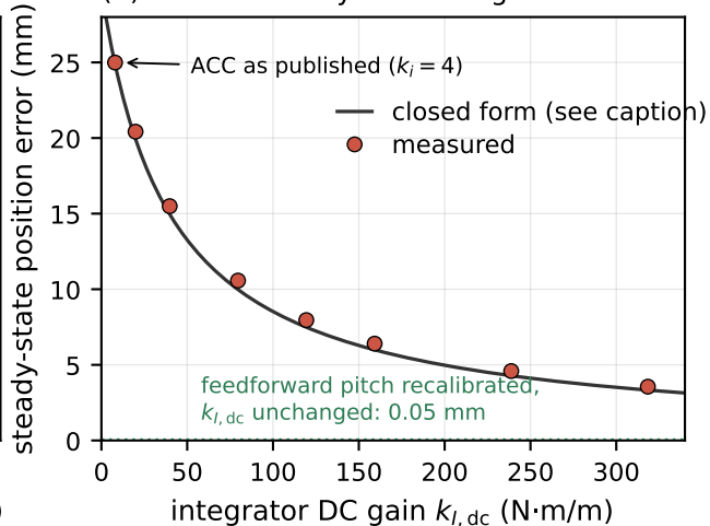
(b) offset is set by finite DC gain
