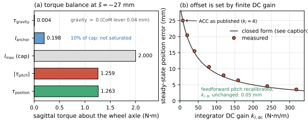
Figure 7: Static torque balance of the sagittal parking offset. (a) Measured sagittal torques at the \bar{s} = -27 mm parking point. The gravity moment about the wheel axle is 0.0040 Nm and the anchor integral sits at 10 % of its clamp, so the offset is neither gravity-driven nor a saturation artifact; the balance is between the pitch and position loops. (b) Steady-state position error against integrator DC gain k_{I,dc} of Eq. (26), swept over k_i \in [4, 160] at fixed leak. The curve is Eq. (27) evaluated with the baseline \tau_{pitch} ; using each run's own measured \tau_{pitch} the closed form tracks all twelve gain and height points to within 0.92 %. The dotted line is the same controller with the feedforward pitch reference recalibrated and k_{I,dc} left unchanged.
