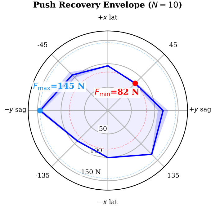
Fig. 4. Omnidirectional push envelope of ACC. This is the same run as row S1 of Table V, not a separate measurement: 8 bearings, N=10 repetitions each, threshold located by binary search over 10 – 160 N to a 5 N tolerance, so the plotted minimum is by construction the F_{\min} of that row. Solid curve: per-bearing mean survivable push magnitude; shaded band: \pm 1 standard deviation over the ten repetitions. The radial axis is linear in force and originates at 0 N, so radial distance is proportional to margin. The envelope is strongly anisotropic, spanning 82.3 – 144.8 N—a 1.8\times ratio between the weakest and strongest bearing. The ordering is -90^\circ ( 144.8 N) > 135^\circ ( 132.2 N) > 90^\circ ( 117.8 N) > -45^\circ ( 107.3 N) > 180^\circ ( 100.7 N) > 0^\circ ( 95.6 N) > -135^\circ ( 91.9 N) > 45^\circ ( 82.3 N). Two regularities are visible. First, the actuated axis is the strong one: bearings are applied in the world frame as \mathbf{f} = F(\cos \theta, \sin \theta, 0) , so \pm 90^\circ are purely sagittal and 0^\circ/180^\circ purely lateral (Sec. V-A). The two sagittal bearings average 131.3 N against 98.2 N for the two lateral ones, a 1.34\times advantage. This is the expected asymmetry for a wheeled biped: sagittally the wheels accelerate the contact patch back under the CoM and convert the impulse into a controlled excursion, whereas laterally no actuator produces ground force at all and the only restoring authority is the static w_{\text{track}} = 0.278 m track width plus hip-roll PD. We compare axis means rather than ranks because the raw ordering is contaminated by the second regularity. Second, the envelope is measurably chiral : 135^\circ survives 40.3 N more than -135^\circ , and -90^\circ 27.0 N more than 90^\circ . This is not sampling noise and not the plant, which is mirror-symmetric to numerical precision: it is the sign convention of the controller's antisymmetric hip-roll and hip-yaw channels, which leaves the closed loop C_2 -equivariant but mirror-broken. The text traces it through the \sin 2\theta harmonic and closes the argument with two control experiments. F_{\min} (red) is the bearing-wise minimum and is the figure of merit quoted throughout the paper, because it is the magnitude survived in every direction; F_{\max} (blue) is shown only to indicate the spread.
