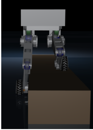
Fig. 6. One-wheel curb (20 cm). With the per-leg height split and the straddle gating of §IV-F: 3.9 \pm 0.1^\circ straddle roll, 10/10 traversed. With a symmetric posture (split removed): the curb-side leg cannot fold far enough, roll diverges past 60^\circ within 0.8 s of curb entry, 0/10.
