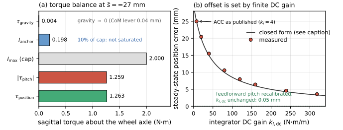
Fig. 7. Static torque balance of the sagittal parking offset. (a) Measured sagittal torques at the \bar{s} = -27 \text{ mm} parking point. The gravity moment about the wheel axle is 0.0040 \text{ Nm} and the anchor integral sits at 10% of its clamp, so the offset is neither gravity-driven nor a saturation artifact; the balance is between the pitch and position loops. (b) Steady-state position error against integrator DC gain k_{I,\text{dc}} of Eq. (26), swept over k_i \in [4, 160] at fixed leak. The curve is Eq. (27) evaluated with the baseline \tau_{\text{pitch}} ; using each run's own measured \tau_{\text{pitch}} the closed form tracks all twelve gain and height points to within 0.92%. The dotted line is the same controller with the feedforward pitch reference recalibrated and k_{I,\text{dc}} left unchanged.
