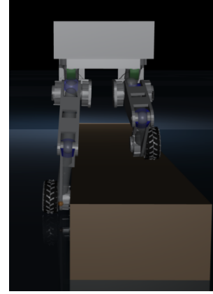
Fig. 6. One-wheel curb (20 cm). With the per-leg height split and the straddling of §IV-F: 3.9 \pm 0.1^\circ straddle roll, 10/10 traversed. With a symmetric posture (split removed): the curb-side leg cannot fold far enough, roll diverges past 60^\circ within 0.8 s of curb entry, 0/10.
