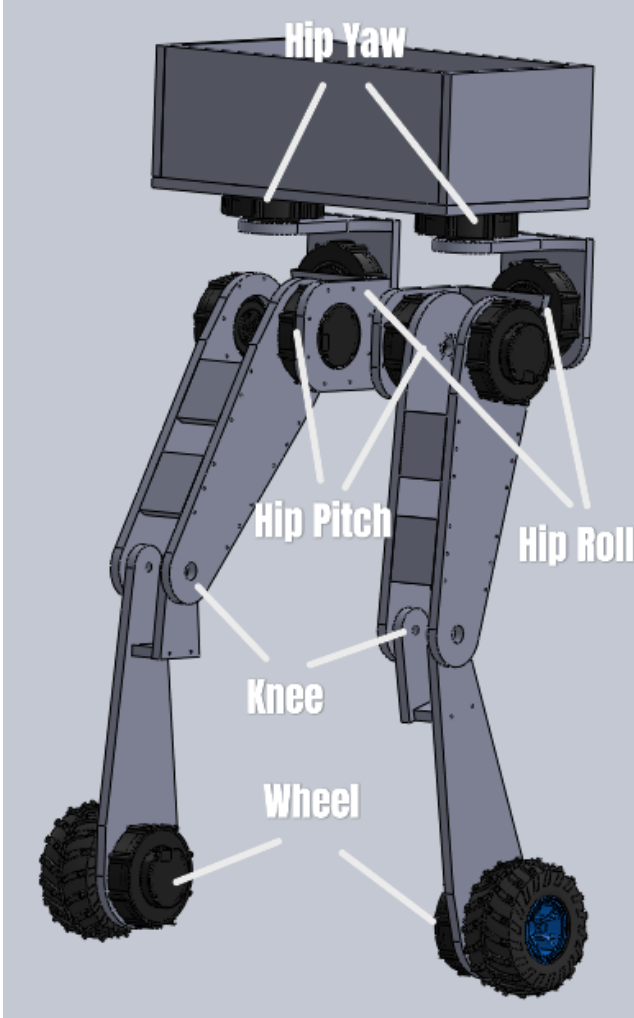
Figure 1: Robot joint layout with world coordinate frame (right-handed, Z up). In the model as built, both wheel axles lie along world X and the two wheel links are separated by 0.271 m along X ; the rolling—and therefore sagittal—direction is world Y , and world X is the lateral (track) axis. All axis-resolved results in this paper follow that convention, verified four independent ways in Section 5.1. The CoM is located at the torso geometric center. Each leg: hip roll (HR), hip yaw (HY), hip pitch (HP), knee (KN), wheel (WH).
