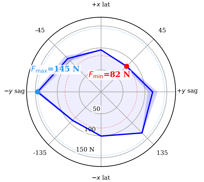
Figure 4: Omnidirectional push envelope of ACC. This is the same run as row S1 of Table 4, not a separate measurement: 8 bearings, N=10 repetitions each, threshold located by binary search over 10–160 N to a 5 N tolerance, so the plotted minimum is by construction the F_{\min} of that row. Solid curve: per-bearing mean survivable push magnitude; shaded band: \pm 1 standard deviation over the ten repetitions. The radial axis is linear in force and originates at 0 N, so radial distance is proportional to margin. The envelope is strongly anisotropic, spanning 82.3–144.8 N—a 1.8× ratio between the weakest and strongest bearing. The ordering is -90^\circ (144.8 N) > 135^\circ (132.2 N) > 90^\circ (117.8 N) > -45^\circ (107.3 N) > 180^\circ (100.7 N) > 0^\circ (95.6 N) > -135^\circ (91.9 N) > 45^\circ (82.3 N). Two regularities are visible. First, the actuated axis is the strong one: bearings are applied in the world frame as \mathbf{f} = F(\cos \theta, \sin \theta, 0) , so \pm 90^\circ are purely sagittal and 0^\circ/180^\circ purely lateral (Section 5.1). The two sagittal bearings average 131.3 N against 98.2 N for the two lateral ones, a 1.34× advantage. This is the expected asymmetry for a wheeled biped: sagittally the wheels accelerate the contact patch back under the CoM and convert the impulse into a controlled excursion, whereas laterally no actuator produces ground force at all and the only restoring authority is the static w_{\text{track}} = 0.278 m track width plus hip-roll PD. We compare axis means rather than ranks because the raw ordering is contaminated by the second regularity. Second, the envelope is measurably chiral : 135^\circ survives 40.3 N more than -135^\circ , and -90^\circ 27.0 N more than 90^\circ . This is not sampling noise and not the plant, which is mirror-symmetric to numerical precision: it is the sign convention of the controller's antisymmetric hip-roll and hip-yaw channels, which leaves the closed loop C_2 -equivariant but mirror-broken. The text traces it through the \sin 2\theta harmonic and closes the argument with two control experiments. F_{\min} (red) is the bearing-wise minimum and is the figure of merit quoted throughout the paper, because it is the magnitude survived in every direction; F_{\max} (blue) is shown only to indicate the spread.
