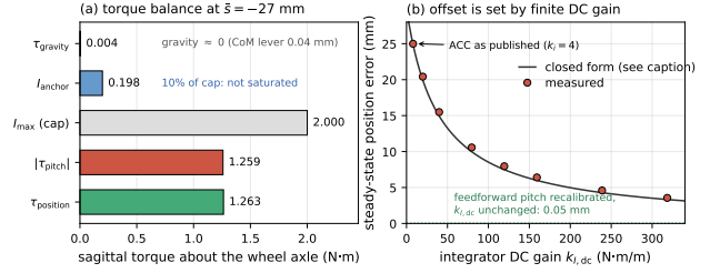
Figure 7: Static torque balance of the sagittal parking offset. (a) Measured sagittal torques at the \bar{s} = -27 \text{ mm} parking point. The gravity moment about the wheel axle is 0.0040 Nm and the anchor integral sits at 10 % of its clamp, so the offset is neither gravity-driven nor a saturation artifact; the balance is between the pitch and position loops. (b) Steady-state position error against integrator DC gain k_{I,\text{dc}} of Eq. (26), swept over k_i \in [4, 160] at fixed leak. The curve is Eq. (27) evaluated with the baseline \tau_{\text{pitch}} ; using each run's own measured \tau_{\text{pitch}} the closed form tracks all twelve gain and height points to within 0.92 %. The dotted line is the same controller with the feedforward pitch reference recalibrated and k_{I,\text{dc}} left unchanged.
