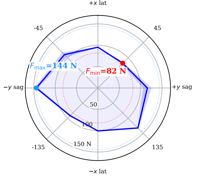
Fig. 4. Omnidirectional push envelope of ACC. This is the same run as row S1 of Table V, not a separate measurement: 8 bearings, threshold located by binary search over 10–160 N to a 5 N tolerance, so the plotted minimum is by construction the F_{\min} of that row. F_{\text{med}} is not read off this figure: it is the per-repetition median over the 8 bearings, averaged over repetitions (108.4 N), which differs from the median of the per-bearing means plotted here (105.6 N) because median and mean do not commute. Solid curve: per-bearing mean survivable push magnitude; shaded band: \pm 1 standard deviation over the 30 repetitions. The radial axis is linear in force and originates at 0 N, so radial distance is proportional to margin. The envelope is strongly anisotropic, spanning 82.1–144.1 N—a 1.8× ratio between the weakest and strongest bearing. The ordering is -90^\circ (144.1 N) > 135^\circ (132.5 N) > 90^\circ (115.8 N) > -45^\circ (110.5 N) > 180^\circ (100.6 N) > 0^\circ (95.5 N) > -135^\circ (91.8 N) > 45^\circ (82.1 N). Two regularities are visible. First, the actuated axis is the strong one: bearings are applied in the world frame as \mathbf{f} = F(\cos \theta, \sin \theta, 0) , so \pm 90^\circ are purely sagittal and 0^\circ/180^\circ purely lateral (Sec. V-A). The two sagittal bearings average 130.0 N against 98.0 N for the two lateral ones, a 1.33× advantage. This is the expected asymmetry for a wheeled biped: sagittally the wheels accelerate the contact patch back under the CoM and convert the impulse into a controlled excursion, whereas laterally no actuator produces ground force at all and the only restoring authority is the static w_{\text{track}} = 0.278 m track width plus hip-roll PD. We compare axis means rather than ranks because the raw ordering is contaminated by the second regularity. Second, the envelope is measurably chiral : 135^\circ survives 40.7 N more than -135^\circ , and -90^\circ 28.3 N more than 90^\circ . This is not sampling noise and not the plant, which is mirror-symmetric to numerical precision: it is the sign convention of the controller’s antisymmetric hip-roll and hip-yaw channels, which leaves the closed loop C_2 -equivariant but mirror-broken. The text traces it through the \sin 2\theta harmonic and closes the argument with two control experiments. F_{\min} (red) is the bearing-wise minimum and is the figure of merit quoted throughout the paper, because it is the magnitude survived in every direction; F_{\max} (blue) is shown only to indicate the spread.
