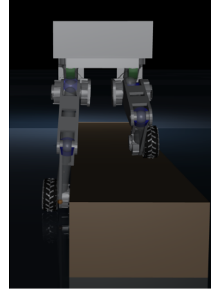
Fig. 6. One-wheel curb (20 cm). With the per-leg height split: 14.9 \pm 0.1^\circ straddle roll, 10/10 settled. With a symmetric posture (split removed): the curb-side leg cannot fold far enough, roll diverges past 60^\circ within 0.8 s of curb entry, 0/10.
