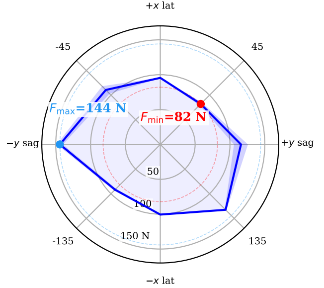
Figure 4: Omnidirectional push envelope of ACC. This is the same run as row S1 of Table 3, not a separate measurement: 8 bearings, threshold located by binary search over 10–160 N to a 5 N tolerance, so the plotted minimum is by construction the F_{\min} of that row. F_{\text{med}} is not read off this figure: it is the per-repetition median over the 8 bearings, averaged over repetitions (108.4 N), which differs from the median of the per-bearing means plotted here (105.6 N) because median and mean do not commute. Solid curve: per-bearing mean survivable push magnitude; shaded band: \pm 1 standard deviation over the 30 repetitions. The radial axis is linear in force and originates at 0 N, so radial distance is proportional to margin. The envelope is strongly anisotropic, spanning 82.1–144.1 N, a 1.8 \times ratio between the weakest and strongest bearing. The ordering is -90^\circ (144.1 N) > 135^\circ (132.5 N) > 90^\circ (115.8 N) > -45^\circ (110.5 N) > 180^\circ (100.6 N) > 0^\circ (95.5 N) > -135^\circ (91.8 N) > 45^\circ (82.1 N). Two regularities are visible. First, the actuated axis is the strong one: bearings are applied in the world frame as \mathbf{f} = F(\cos \theta, \sin \theta, 0) , so \pm 90^\circ are purely sagittal and 0^\circ/180^\circ purely lateral (Section 5.1). The two sagittal bearings average 130.0 N against 98.0 N for the two lateral ones, a 1.33 \times advantage. This is the expected asymmetry for a wheeled biped: sagittally the wheels accelerate the contact patch back under the CoM and convert the impulse into a controlled excursion, whereas laterally no actuator produces ground force at all and the only restoring authority is the static w_{\text{track}} = 0.278 m track width plus hip-roll PD. We compare axis means rather than ranks because the raw ordering is contaminated by the second regularity. Second, the envelope is measurably chiral : 135^\circ survives 40.7 N more than -135^\circ , and -90^\circ 28.3 N more than 90^\circ . This is not sampling noise and not the plant, which is mirror-symmetric to numerical precision: it is the sign convention of the controller's antisymmetric hip-roll and hip-yaw channels, which leaves the closed loop C_2 -equivariant but mirror-broken. The text traces it through the \sin 2\theta harmonic and closes the argument with two control experiments. F_{\min} (red) is the bearing-wise minimum and is the figure of merit quoted throughout the paper, because it is the magnitude survived in every direction; F_{\max} (blue) is shown only to indicate the spread.
