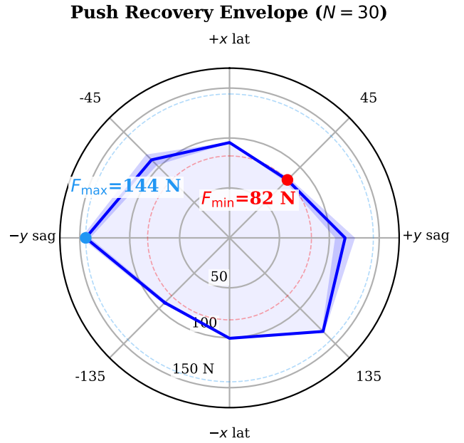
Figure 4: Omnidirectional push envelope of ACC. This is the same run as row S1 of Table 5, not a separate measurement: 8 bearings, threshold located by binary search over 10\text{--}160\text{ N} to a 5\text{ N} tolerance, so the plotted minimum is by construction the F_{\min} of that row. F_{\text{med}} is not read off this figure: it is the per-repetition median over the 8 bearings, averaged over repetitions ( 108.4\text{ N} ), which differs from the median of the per-bearing means plotted here ( 105.6\text{ N} ) because median and mean do not commute. Solid curve: per-bearing mean survivable push magnitude; shaded band: \pm 1 standard deviation over the 30 repetitions. The radial axis is linear in force and originates at 0\text{ N} , so radial distance is proportional to margin. The envelope is strongly anisotropic, spanning 82.1\text{--}144.1\text{ N} , a 1.8\times ratio between the weakest and strongest bearing. The ordering is -90^\circ (144.1\text{ N}) > 135^\circ (132.5\text{ N}) > 90^\circ (115.8\text{ N}) > -45^\circ (110.5\text{ N}) > 180^\circ (100.6\text{ N}) > 0^\circ (95.5\text{ N}) > -135^\circ (91.8\text{ N}) > 45^\circ (82.1\text{ N}) . Two regularities are visible. First, the actuated axis is the strong one: bearings are applied in the world frame as \mathbf{f} = F(\cos \theta, \sin \theta, 0) , so \pm 90^\circ are purely sagittal and 0^\circ/180^\circ purely lateral (Section 5.1). The two sagittal bearings average 130.0\text{ N} against 98.0\text{ N} for the two lateral ones, a 1.33\times advantage. This is the expected asymmetry for a wheeled biped: sagittally the wheels accelerate the contact patch back under the CoM and convert the impulse into a controlled excursion, whereas laterally no actuator produces ground force at all and the only restoring authority is the static w_{\text{track}} = 0.278\text{ m} track width plus hip-roll PD. We compare axis means rather than ranks because the raw ordering is contaminated by the second regularity. Second, the envelope is measurably chiral : 135^\circ survives 40.7\text{ N} more than -135^\circ , and -90^\circ 28.3\text{ N} more than 90^\circ . This is not sampling noise and not the plant, which is mirror-symmetric to numerical precision: it is the sign convention of the controller's antisymmetric hip-roll and hip-yaw channels, which leaves the closed loop C_2 -equivariant but mirror-broken. The text traces it through the \sin 2\theta harmonic and closes the argument with two control experiments. F_{\min} (red) is the bearing-wise minimum and is the figure of merit quoted throughout the paper, because it is the magnitude survived in every direction; F_{\max} (blue) is shown only to indicate the spread.
