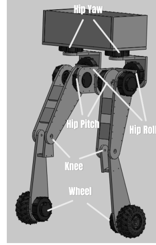
Figure 1. Robot joint layout with world frame (right-handed, Z up). Wheel axles lie along world X, so the rolling (and therefore sagittal) direction is world Y and world X is the lateral (track) axis. Each leg: hip roll (HR), hip yaw (HY), hip pitch (HP), knee (KN), wheel (WH).
