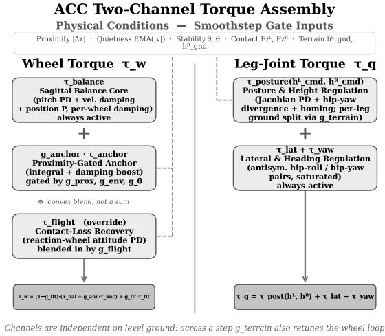
Figure 2. ACC two-channel torque assembly. Physical conditions gate each component via continuous smoothstep functions (dashed). The latched flight gate overrides the wheel channel rather than adding to it, and per-leg ground adaptation enters as a split pair of height references, not an added torque.
