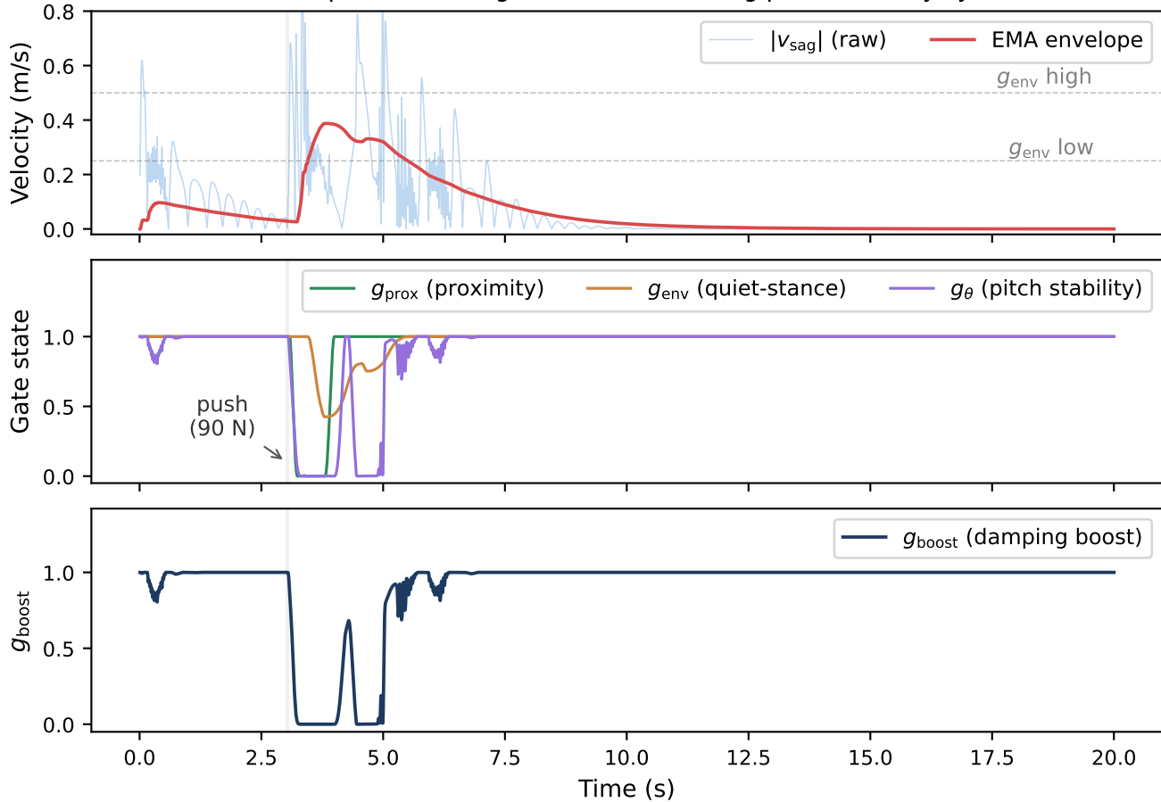
Envelope follower + gate activation during push-recovery cycle
