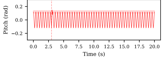
Fig. 4. Post-push pitch ringdown: ACC (top) vs. P-only (bottom). 90 N push applied at t = 3 s. ACC ringdown completes in \sim 9 s; P-only oscillation persists indefinitely due to equilibrium bias.
