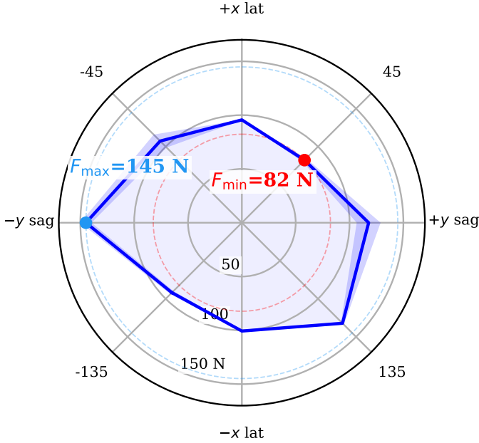
Fig. 4. Omnidirectional push envelope of ACC. This is the same run as row S1 of Table IV, not a separate measurement: 8 bearings, N=10 repetitions each, threshold located by binary search over 10–160 N to a 5 N tolerance, so the plotted minimum is by construction the F_{\min} of that row. Solid curve: per-bearing mean survivable push magnitude; shaded band: \pm 1 standard deviation over the ten repetitions. The radial axis is linear in force and originates at 0 N, so radial distance is proportional to margin. The envelope is strongly anisotropic, spanning 82.3–144.8 N—a 1.8\times ratio between the weakest and strongest bearing. The ordering is -90^\circ (144.8 N) > 135^\circ (132.2 N) > 90^\circ (117.8 N) > -45^\circ (107.3 N) > 180^\circ (100.7 N) > 0^\circ (95.6 N) > -135^\circ (91.9 N) > 45^\circ (82.3 N). Two regularities are visible. First, the actuated axis is the strong one: bearings are applied in the world frame as \mathbf{f} = F(\cos \theta, \sin \theta, 0) , so \pm 90^\circ are purely sagittal and 0^\circ/180^\circ purely lateral (Sec. V-A). The two sagittal bearings average 131.3 N against 98.2 N for the two lateral ones, a 1.34\times advantage. This is the expected asymmetry for a wheeled biped: sagittally the wheels accelerate the contact patch back under the CoM and convert the impulse into a controlled excursion, whereas laterally no actuator produces ground force at all and the only restoring authority is the static w_{\text{track}} = 0.278 m track width plus hip-roll PD. We compare axis means rather than ranks because the raw ordering is contaminated by the second regularity. Second, the envelope is measurably chiral : 135^\circ survives 40.3 N more than -135^\circ , and -90^\circ 27.0 N more than 90^\circ . This is not sampling noise and not the plant, which is mirror-symmetric to numerical precision: it is the sign convention of the controller’s antisymmetric hip-roll and hip-yaw channels, which leaves the closed loop C_2 -equivariant but mirror-broken. The text traces it through the \sin 2\theta harmonic and closes the argument with two control experiments. F_{\min} (red) is the bearing-wise minimum and is the figure of merit quoted throughout the paper, because it is the magnitude survived in every direction; F_{\max} (blue) is shown only to indicate the spread.
