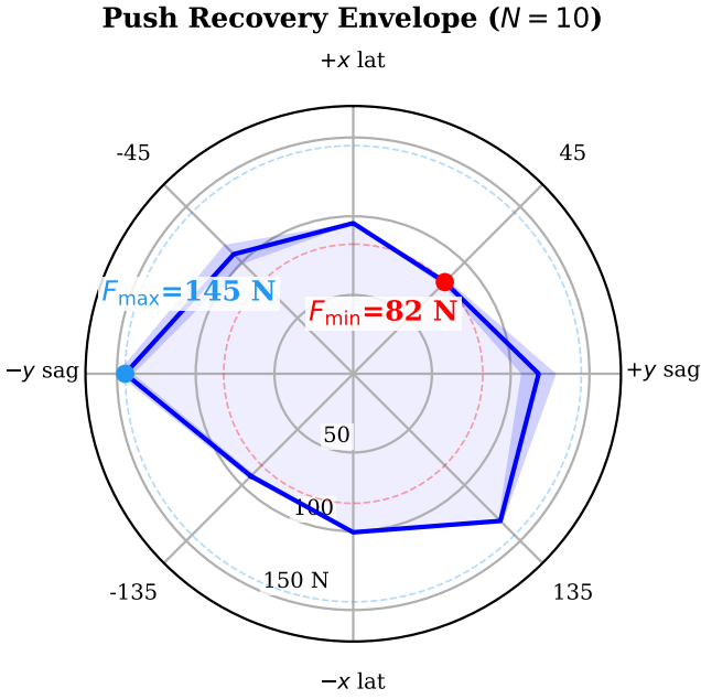
Figure 4: Omnidirectional push envelope of ACC. This is the same run as row S1 of Table 5, not a separate measurement: 8 bearings, threshold located by binary search over 10–160 N to a 5 N tolerance, so the plotted minimum is by construction the F_{\min} of that row. It is drawn at N=10 , the first ten seeds of that row's 30; extending to all 30 moves each per-bearing mean by at most 3.3 N and F_{\min} by 0.2 N, so the envelope below is plotted on the smaller set rather than re-rendered. Solid curve: per-bearing mean survivable push magnitude; shaded band: \pm 1 standard deviation over the ten repetitions. The radial axis is linear in force and originates at 0 N, so radial distance is proportional to margin. The envelope is strongly anisotropic, spanning 82.3–144.8 N—a 1.8 \times ratio between the weakest and strongest bearing. The ordering is -90^\circ (144.8 N) > 135^\circ (132.2 N) > 90^\circ (117.8 N) > -45^\circ (107.3 N) > 180^\circ (100.7 N) > 0^\circ (95.6 N) > -135^\circ (91.9 N) > 45^\circ (82.3 N). Two regularities are visible. First, the actuated axis is the strong one: bearings are applied in the world frame as \mathbf{f} = F(\cos \theta, \sin \theta, 0) , so \pm 90^\circ are purely sagittal and 0^\circ/180^\circ purely lateral (Section 5.1). The two sagittal bearings average 131.3 N against 98.2 N for the two lateral ones, a 1.34 \times advantage. This is the expected asymmetry for a wheeled biped: sagittally the wheels accelerate the contact patch back under the CoM and convert the impulse into a controlled excursion, whereas laterally no actuator produces ground force at all and the only restoring authority is the static w_{\text{track}} = 0.278 m track width plus hip-roll PD. We compare axis means rather than ranks because the raw ordering is contaminated by the second regularity. Second, the envelope is measurably chiral : 135^\circ survives 40.3 N more than -135^\circ , and -90^\circ 27.0 N more than 90^\circ . This is not sampling noise and not the plant, which is mirror-symmetric to numerical precision: it is the sign convention of the controller's antisymmetric hip-roll and hip-yaw channels, which leaves the closed loop C_2 -equivariant but mirror-broken. The text traces it through the \sin 2\theta harmonic and closes the argument with two control experiments. F_{\min} (red) is the bearing-wise minimum and is the figure of merit quoted throughout the paper, because it is the magnitude survived in every direction; F_{\max} (blue) is shown only to indicate the spread.
