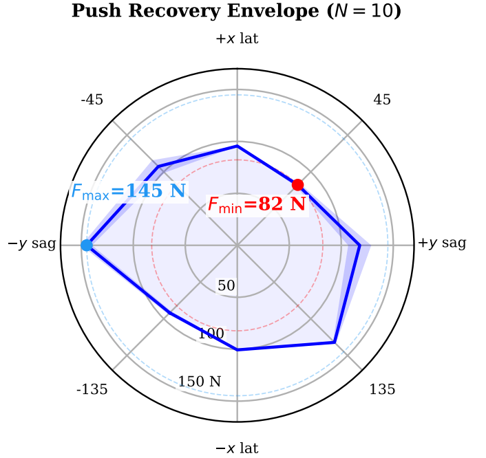
Fig. 4. Omnidirectional push envelope of ACC. This is the same run as row S1 of Table V, not a separate measurement: 8 bearings, threshold located by binary search over 10–160 N to a 5 N tolerance, so the plotted minimum is by construction the F_{\min} of that row. It is drawn at N=10 , the first ten seeds of that row's 30; extending to all 30 moves each per-bearing mean by at most 3.3 N and F_{\min} by 0.2 N, so the envelope below is plotted on the smaller set rather than re-rendered. Solid curve: per-bearing mean survivable push magnitude; shaded band: \pm 1 standard deviation over the ten repetitions. The radial axis is linear in force and originates at 0 N, so radial distance is proportional to margin. The envelope is strongly anisotropic, spanning 82.3–144.8 N—a 1.8\times ratio between the weakest and strongest bearing. The ordering is -90^\circ (144.8 N) > 135^\circ (132.2 N) > 90^\circ (117.8 N) > -45^\circ (107.3 N) > 180^\circ (100.7 N) > 0^\circ (95.6 N) > -135^\circ (91.9 N) > 45^\circ (82.3 N). Two regularities are visible. First, the actuated axis is the strong one: bearings are applied in the world frame as \mathbf{f} = F(\cos \theta, \sin \theta, 0) , so \pm 90^\circ are purely sagittal and 0^\circ/180^\circ purely lateral (Sec. V-A). The two sagittal bearings average 131.3 N against 98.2 N for the two lateral ones, a 1.34\times advantage. This is the expected asymmetry for a wheeled biped: sagittally the wheels accelerate the contact patch back under the CoM and convert the impulse into a controlled excursion, whereas laterally no actuator produces ground force at all and the only restoring authority is the static w_{\text{track}} = 0.278 m track width plus hip-roll PD. We compare axis means rather than ranks because the raw ordering is contaminated by the second regularity. Second, the envelope is measurably chiral : 135^\circ survives 40.3 N more than -135^\circ , and -90^\circ 27.0 N more than 90^\circ . This is not sampling noise and not the plant, which is mirror-symmetric to numerical precision: it is the sign convention of the controller's antisymmetric hip-roll and hip-yaw channels, which leaves the closed loop C_2 -equivariant but mirror-broken. The text traces it through the \sin 2\theta harmonic and closes the argument with two control experiments. F_{\min} (red) is the bearing-wise minimum and is the figure of merit quoted throughout the paper, because it is the magnitude survived in every direction; F_{\max} (blue) is shown only to indicate the spread.
