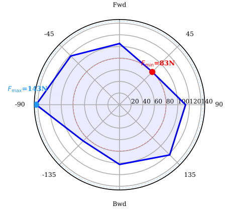
Fig. 4. Omnidirectional push envelope. F_{\min} (red), F_{\max} (blue) across 8 directions.
