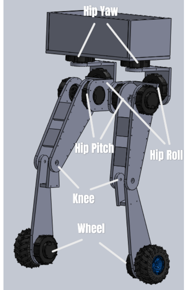
Figure 1. Robot joint layout with world coordinate frame (right-handed, Z up). In the model as built, both wheel axles lie along world X and the two wheel links are separated by 0.271 m along X; the rolling—and therefore sagittal—direction is world Y, and world X is the lateral (track) axis. All axis-resolved results in this paper follow that convention, verified four independent ways in Sec. 5.1. The CoM is located at the torso geometric center. Each leg: hip roll (HR), hip yaw (HY), hip pitch (HP), knee (KN), wheel (WH).
