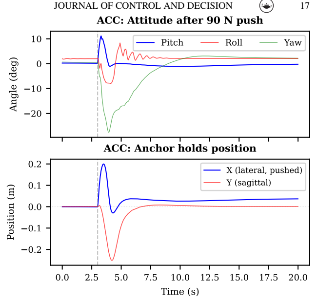
Figure 5. Post-push recovery (90 N lateral, world +x , at t=3 \text{ s} ). Top: attitude angles; stabilization within 2 s. Bottom: planar CoM position, which separates the two axes cleanly. The lateral push couples through roll into a large sagittal excursion ( -251 \text{ mm} peak); the anchor drives that axis back to 1.37 \text{ mm} of home and holds it there at 0.018 \text{ mm} SD over the final 2 s—a 99.5 % recovery. On the pushed lateral axis, which has no actuator authority (Sec. 5.1), the 200 \text{ mm} peak excursion decays only to a permanent 36.2 \text{ mm} offset, 18 % of the peak. The contrast between the two traces is the clearest single illustration of what the anchor does and where it does not act.
