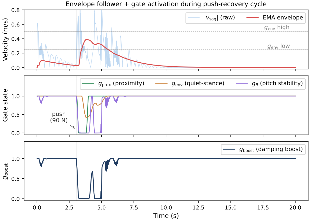
Figure 3. Gate activation during a 90 N lateral (world +x ) push-recovery cycle (100 Hz control). Top: |v_{\text{sag}}| and asymmetric EMA envelope; dashed lines mark the 0.25–0.50 m/s quiet-stance band. Middle: Individual gate states. Bottom: Composite damping boost g_{\text{boost}} . Grey shading: 7-step push window. The three panels are the empirical basis for finding (iii) of §5.1.4: g_{\text{prox}} and g_{\text{env}} both sit pinned at their quiet-stance values before the impulse and after the ringdown, which is why ablating either reproduces ACC bit-for-bit at idle, and why only a disturbance experiment can measure their contribution.
