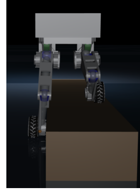
Figure 6. One-wheel curb (20 cm). With the per-leg height split: 14.9 \pm 0.1^\circ straddle roll, 10/10 settled. With a symmetric posture (split removed): the curb-side leg cannot fold far enough, roll diverges past 60^\circ within 0.8 s of curb entry, 0/10.
