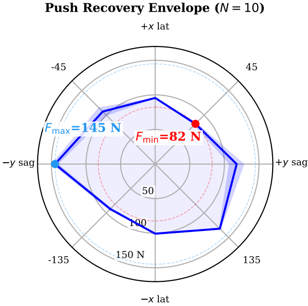
Figure 4: Omnidirectional push envelope of ACC. This is the same run as row S1 of Table 5, not a separate measurement: 8 bearings, N=10 repetitions each, threshold located by binary search over 10–160 N to a 5 N tolerance, so the plotted minimum is by construction the F_{\min} of that row. Solid curve: per-bearing mean survivable push magnitude; shaded band: \pm 1 standard deviation over the ten repetitions. The radial axis is linear in force and originates at 0 N, so radial distance is proportional to margin. The envelope is strongly anisotropic, spanning 82.3–144.8 N—a 1.8 \times ratio between the weakest and strongest bearing. The ordering is -90^\circ (144.8 N) > 135^\circ (132.2 N) > 90^\circ (117.8 N) > -45^\circ (107.3 N) > 180^\circ (100.7 N) > 0^\circ (95.6 N) > -135^\circ (91.9 N) > 45^\circ (82.3 N). Two regularities are visible. First, the actuated axis is the strong one: bearings are applied in the world frame as \mathbf{f} = F(\cos \theta, \sin \theta, 0) , so \pm 90^\circ are purely sagittal and 0^\circ/180^\circ purely lateral (Section 5.1). The two sagittal bearings average 131.3 N against 98.2 N for the two lateral ones, a 1.34 \times advantage. This is the expected asymmetry for a wheeled biped: sagittally the wheels accelerate the contact patch back under the CoM and convert the impulse into a controlled excursion, whereas laterally no actuator produces ground force at all and the only restoring authority is the static w_{\text{track}} = 0.278 m track width plus hip-roll PD. We compare axis means rather than ranks because the raw ordering is contaminated by the second regularity. Second, the envelope is measurably chiral : 135^\circ survives 40.3 N more than -135^\circ , and -90^\circ 27.0 N more than 90^\circ . This is not sampling noise and not the plant, which is mirror-symmetric to numerical precision: it is the sign convention of the controller’s antisymmetric hip-roll and hip-yaw channels, which leaves the closed loop C_2 -equivariant but mirror-broken. The text traces it through the \sin 2\theta harmonic and closes the argument with two control experiments. F_{\min} (red) is the bearing-wise minimum and is the figure of merit quoted throughout the paper, because it is the magnitude survived in every direction; F_{\max} (blue) is shown only to indicate the spread.
