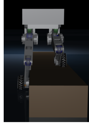
Figure 6: One-wheel curb (20 cm). With the per-leg height split and the straddle gating of Section 4.6: 3.9 \pm 0.1^\circ straddle roll, 10/10 traversed. With a symmetric posture (split removed): the curb-side leg cannot fold far enough, roll diverges past 60^\circ within 0.8 s of curb entry, 0/10.
