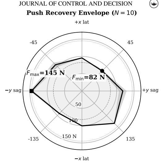
Figure 3. Omnidirectional push envelope of ACC—the same run as row S1 of Table 3. Solid curve: per-bearing mean survivable push over N=10 repetitions; shaded band \pm 1 SD; radial axis linear in force from 0 N. The envelope spans 82.3–144.8 N and is both anisotropic and chiral.
