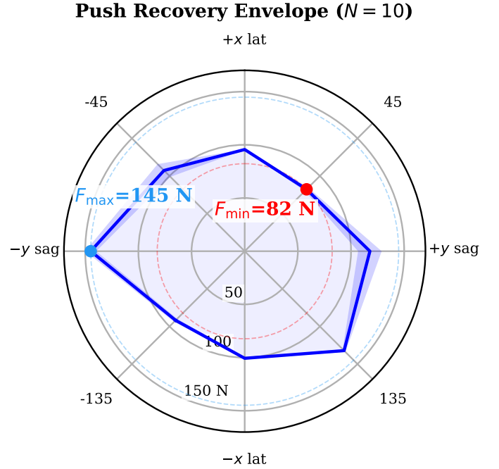
Fig. 4. Omnidirectional push envelope of ACC. This is the same run as row S1 of Table V, not a separate measurement: 8 bearings, N=10 repetitions each, threshold located by binary search over 10–160 N to a 5 N tolerance, so the plotted minimum is by construction the F_{\min} of that row. Solid curve: per-bearing mean survivable push magnitude; shaded band: \pm 1 standard deviation over the ten repetitions. The radial axis is linear in force and originates at 0 N, so radial distance is proportional to margin. The envelope is strongly anisotropic, spanning 82.3–144.8 N—a 1.8\times ratio between the weakest and strongest bearing. The ordering is -90^\circ ( 144.8 N) > 135^\circ ( 132.2 N) > 90^\circ ( 117.8 N) > -45^\circ ( 107.3 N) > 180^\circ ( 100.7 N) > 0^\circ ( 95.6 N) > -135^\circ ( 91.9 N) > 45^\circ ( 82.3 N). Two regularities are visible. First, the actuated axis is the strong one: bearings are applied in the world frame as \mathbf{f} = F(\cos \theta, \sin \theta, 0) , so \pm 90^\circ are purely sagittal and 0^\circ/180^\circ purely lateral (Sec. V-A). The two sagittal bearings average 131.3 N against 98.2 N for the two lateral ones, a 1.34\times advantage. This is the expected asymmetry for a wheeled biped: sagittally the wheels accelerate the contact patch back under the CoM and convert the impulse into a controlled excursion, whereas laterally no actuator produces ground force at all and the only restoring authority is the static w_{\text{track}} = 0.278 m track width plus hip-roll PD. We compare axis means rather than ranks because the raw ordering is contaminated by the second regularity. Second, the envelope is measurably chiral : 135^\circ survives 40.3 N more than -135^\circ , and -90^\circ 27.0 N more than 90^\circ . This is not sampling noise and not the plant, which is mirror-symmetric to numerical precision: it is the sign convention of the controller's antisymmetric hip-roll and hip-yaw channels, which leaves the closed loop C_2 -equivariant but mirror-broken. The text traces it through the \sin 2\theta harmonic and closes the argument with two control experiments. F_{\min} (red) is the bearing-wise minimum and is the figure of merit quoted throughout the paper, because it is the magnitude survived in every direction; F_{\max} (blue) is shown only to indicate the spread.
