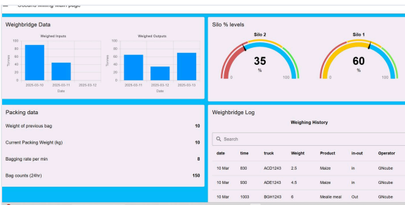
REAL-TIME IIOT WEIGHBRIDGE DASHBOARD
