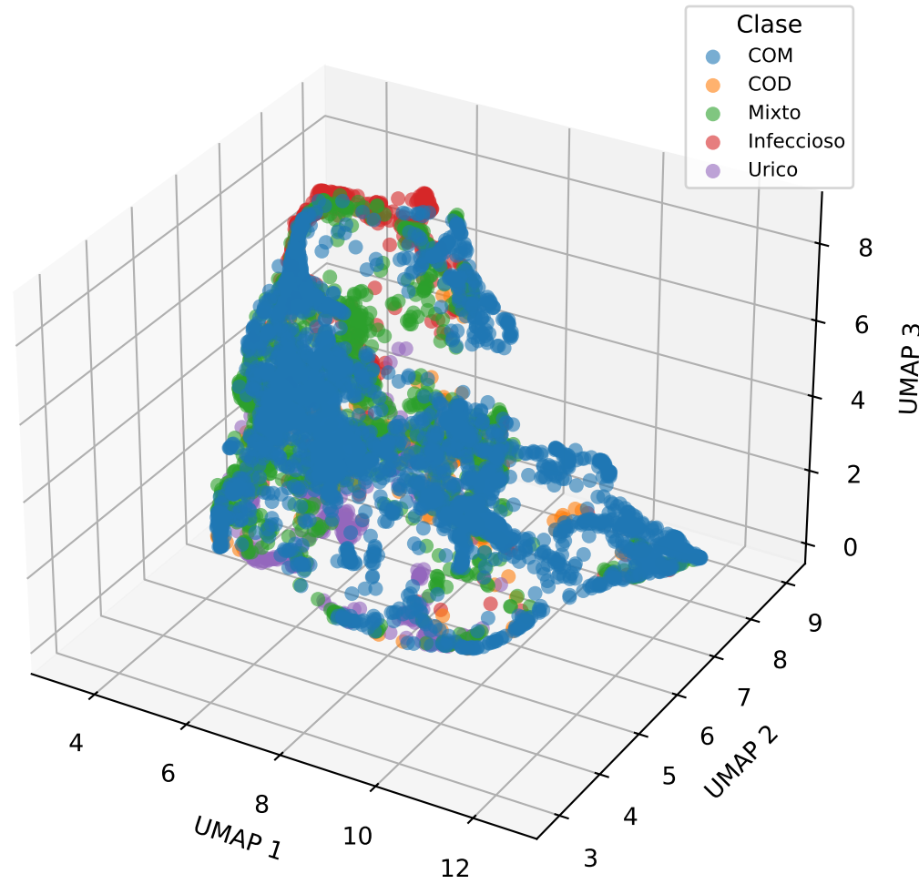
LBP+HSV (40-d)
