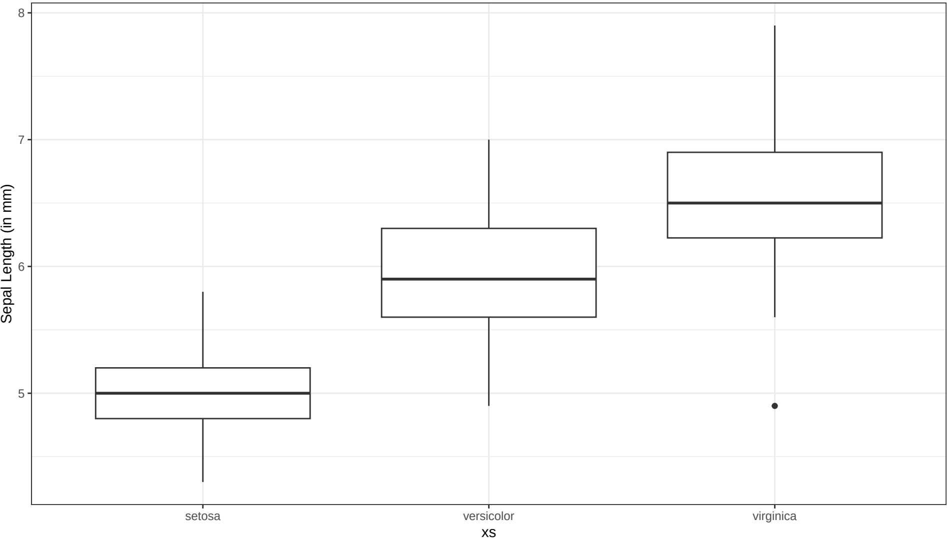
Sepal length by species
