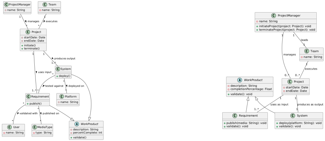
Figure 2-15. Class diagram
