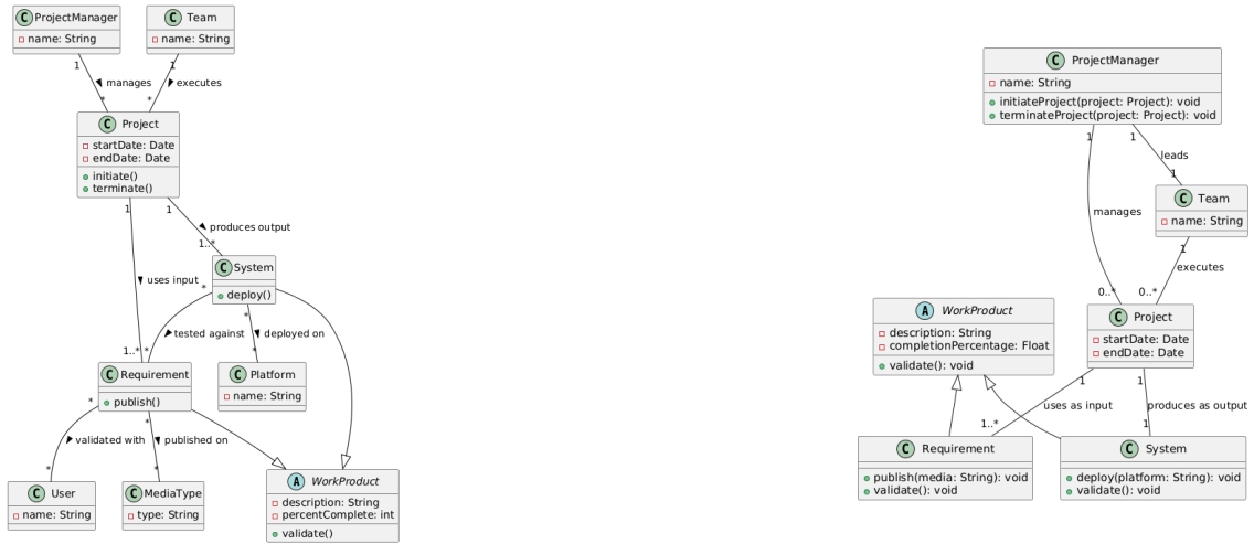
Figure 2-15. Class diagram
