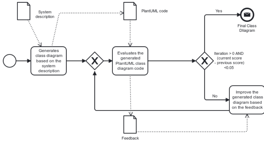
Figure 5.7: Self-refinement loop architecture.
