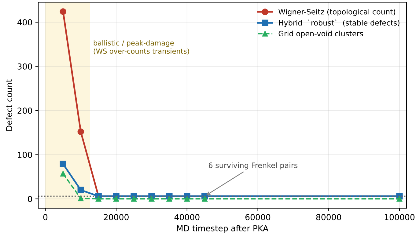
FeCrNi 5 keV cascade — vacancy estimators vs. regime
