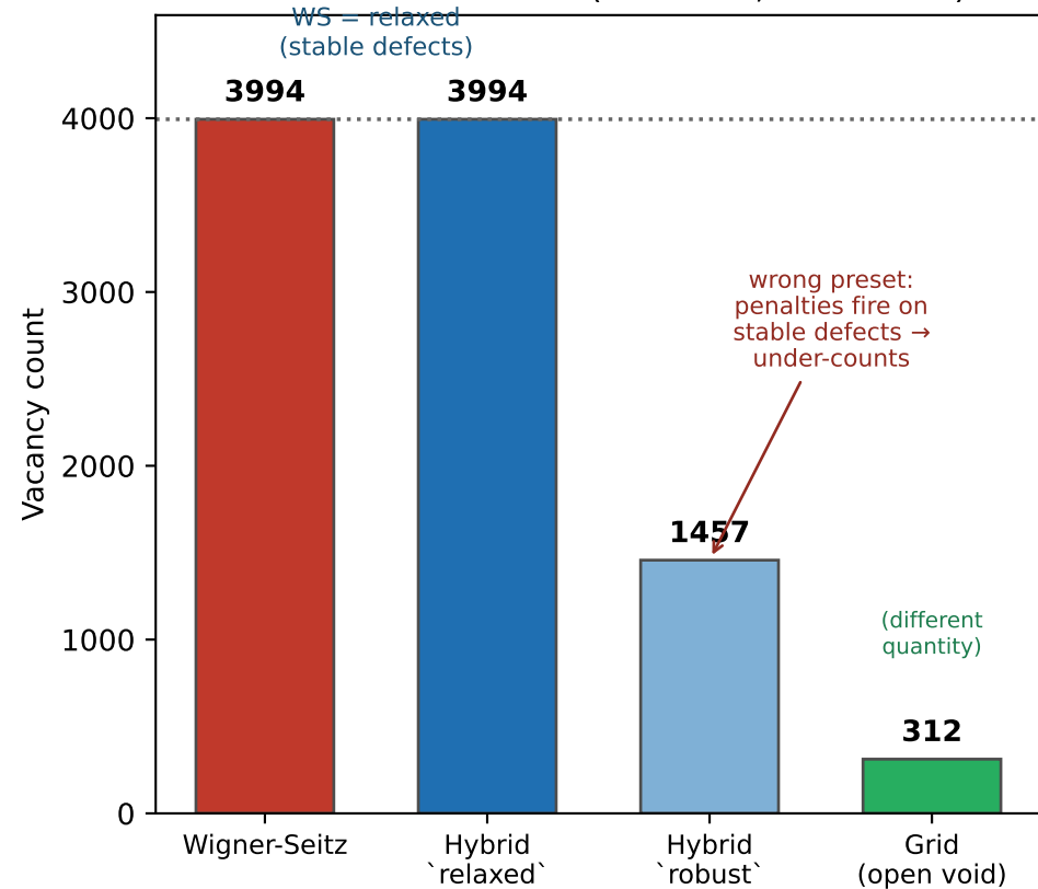
Relaxed FeCrNi HEA (finalCool, t=160000)
