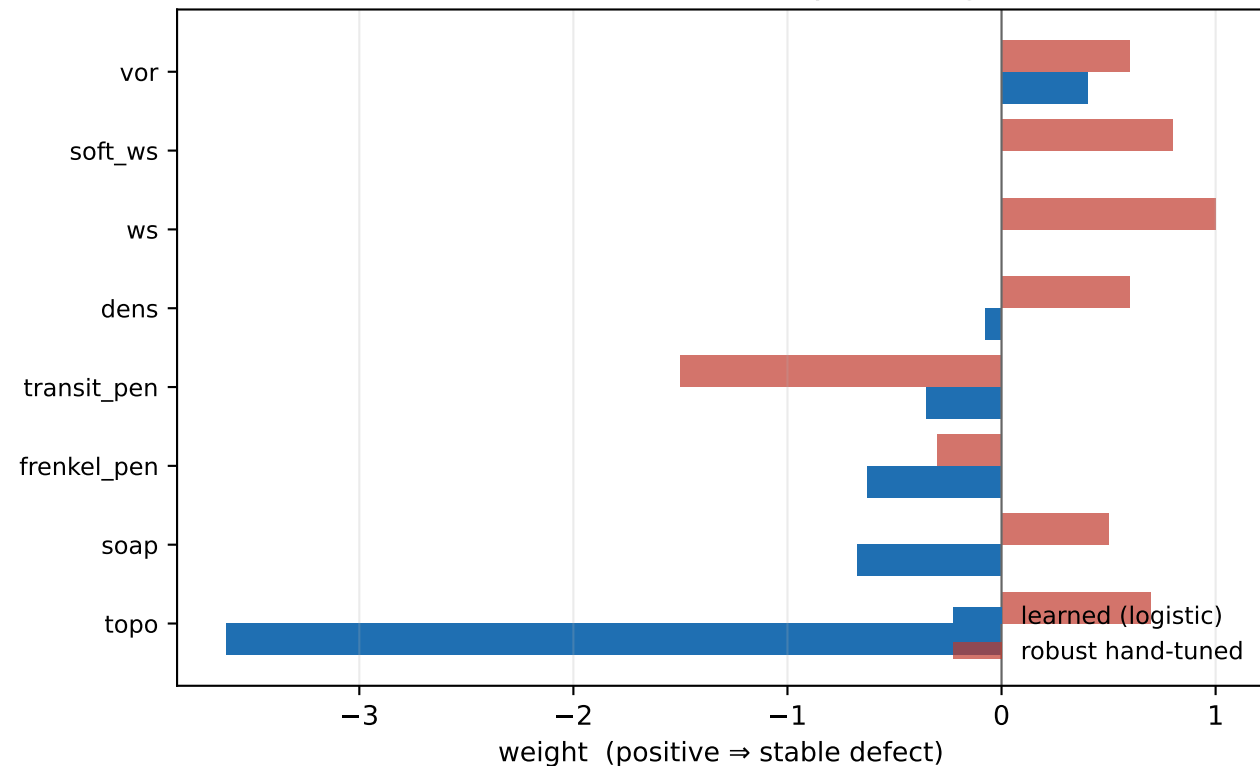
Learned vs hand-tuned hybrid weights
