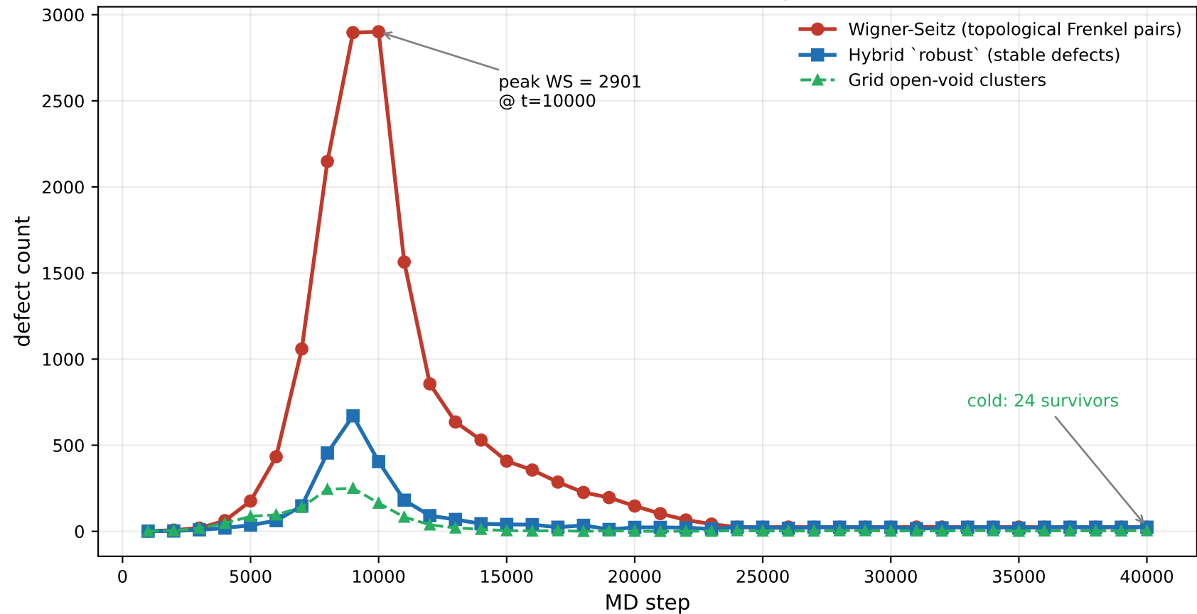
FeCrNi 10kev PKA cascade — damage evolution
