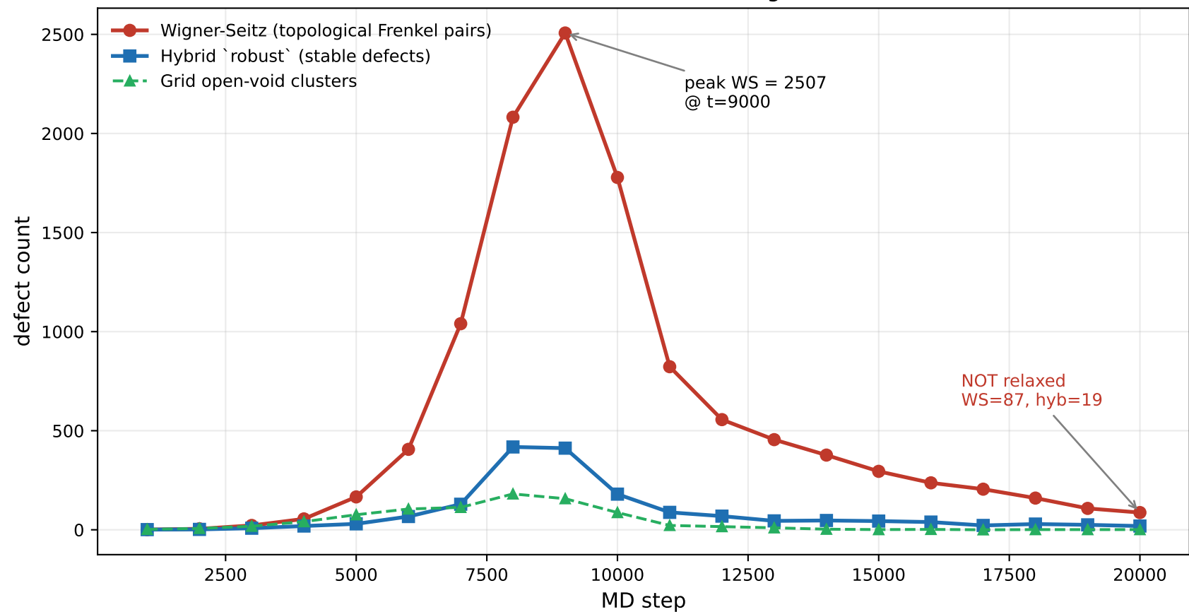
FeCrNi 9kev PKA cascade — damage evolution
