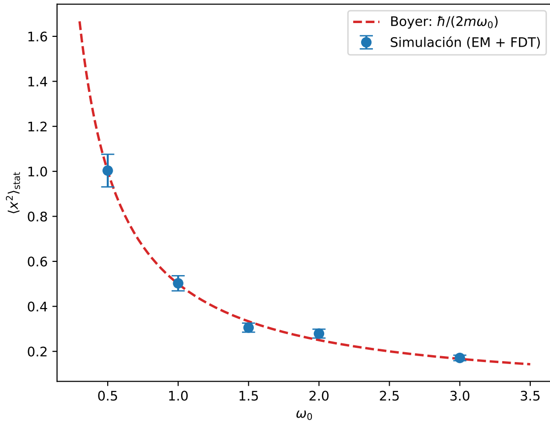
\langle x^2 \rangle = \hbar/(2m\omega_0) — Boyer (1975)
