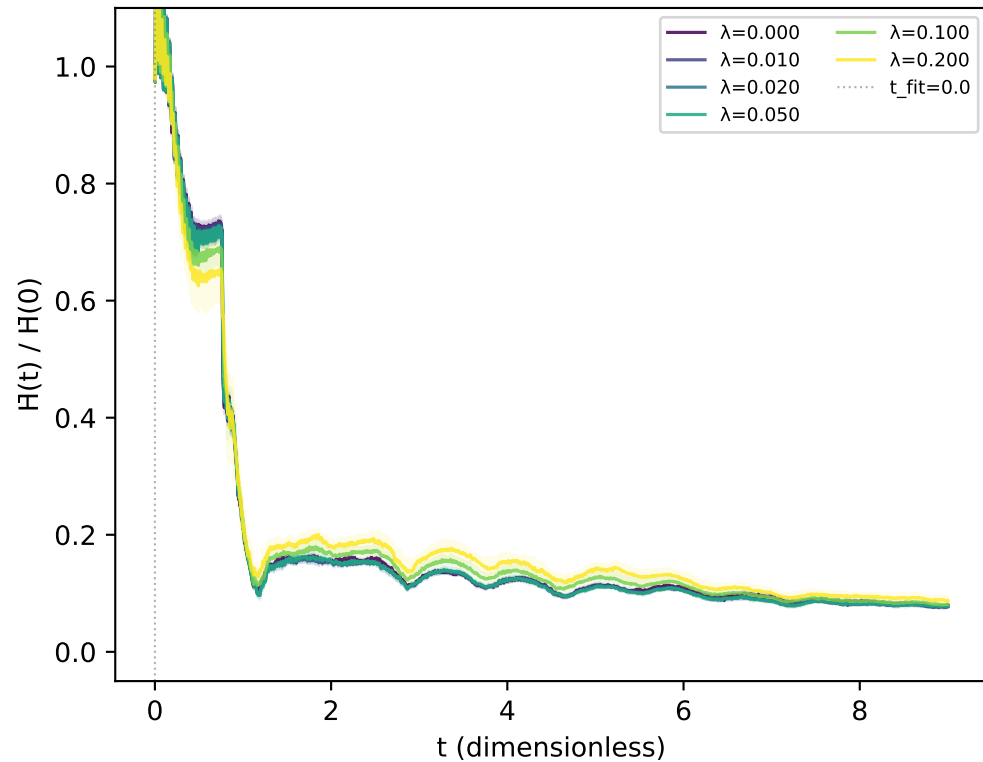
H-function evolution
