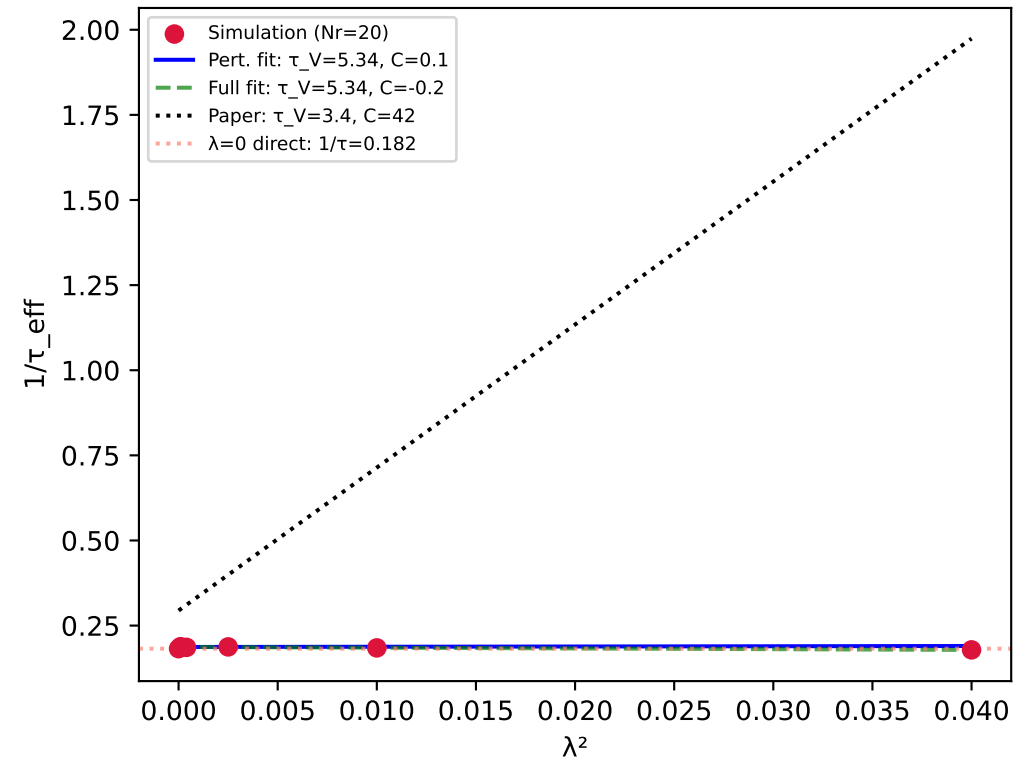
Relaxation rate vs coupling (cf. Fig. 3 paper)
