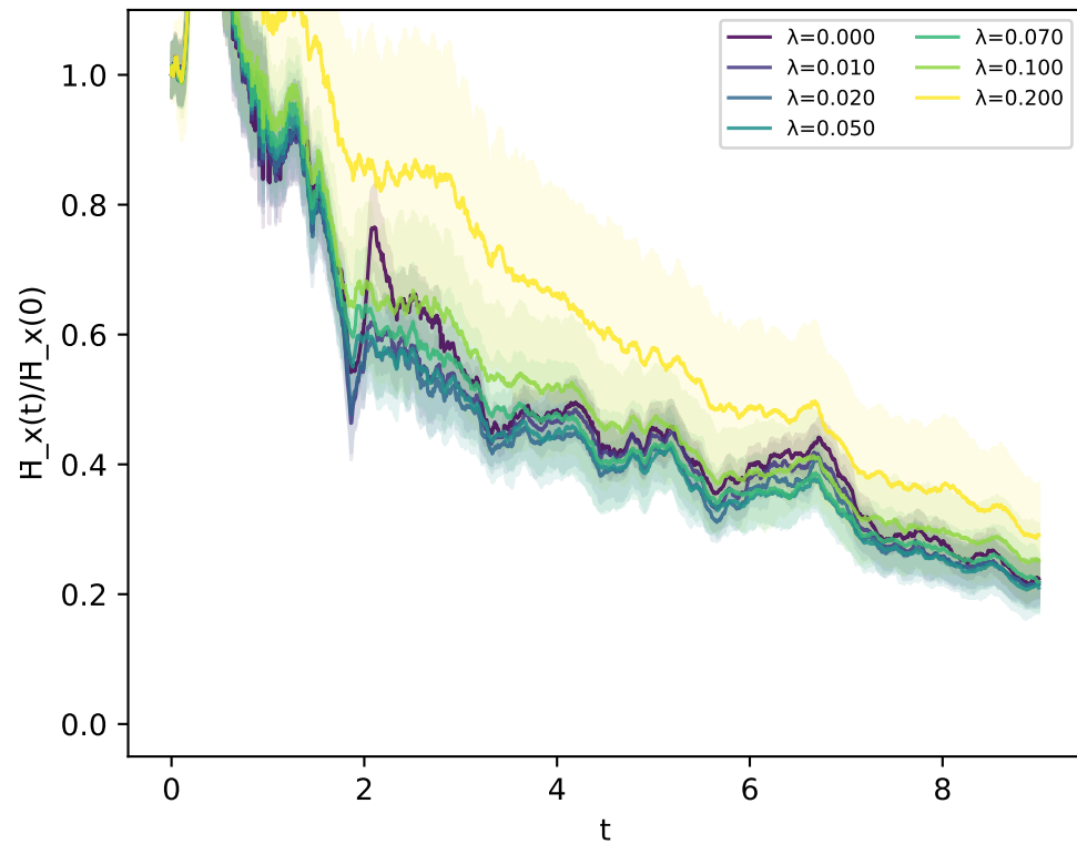
H-function evolution (1D x-marginal)
