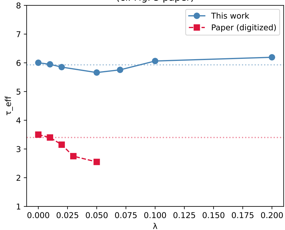
Relaxation time vs coupling (cf. Fig. 3 paper)
