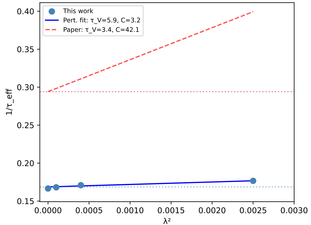
Relaxation rate vs coupling (cf. Fig. 3 right)
