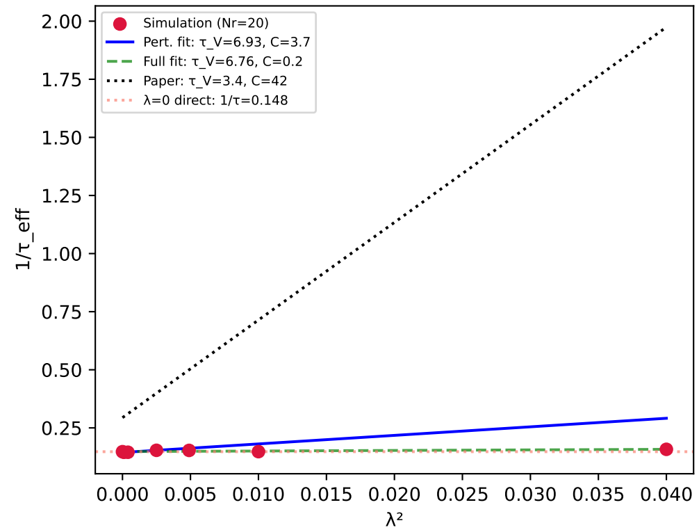
Relaxation rate vs coupling (cf. Fig. 3 paper)
