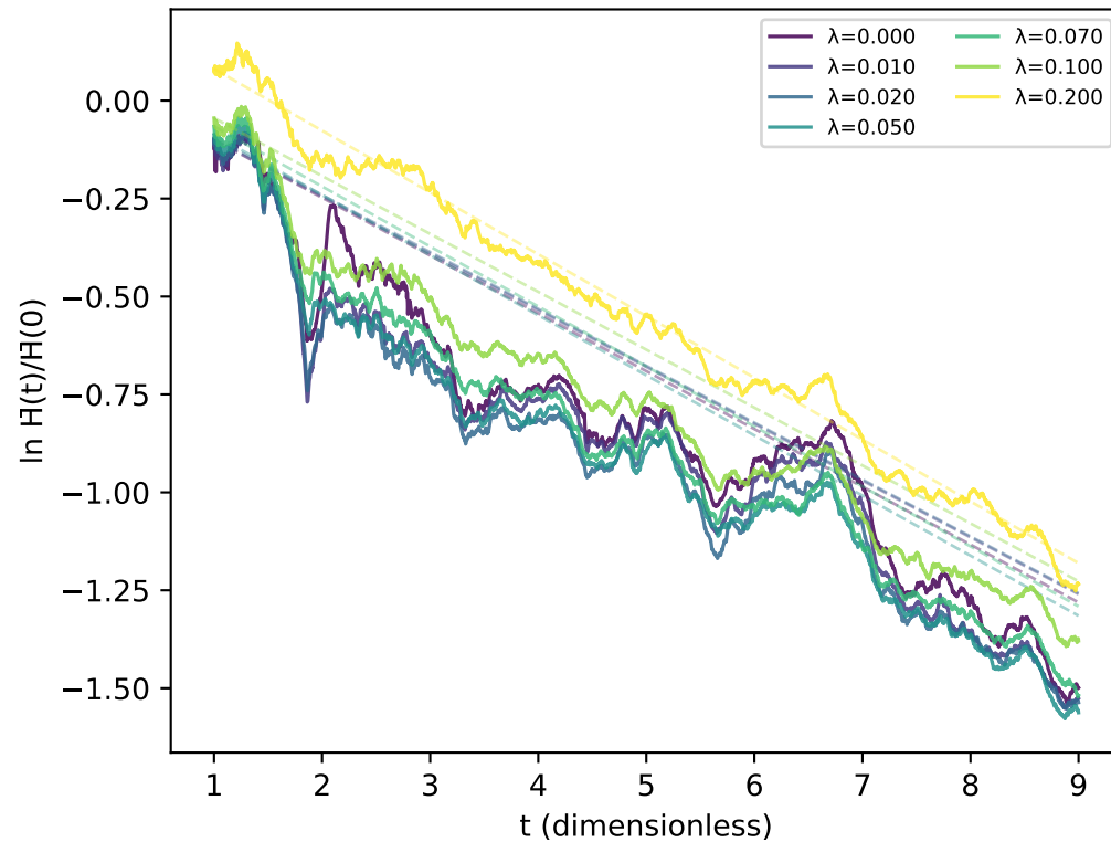
Exponential decay (cf. Fig. 2 paper)
