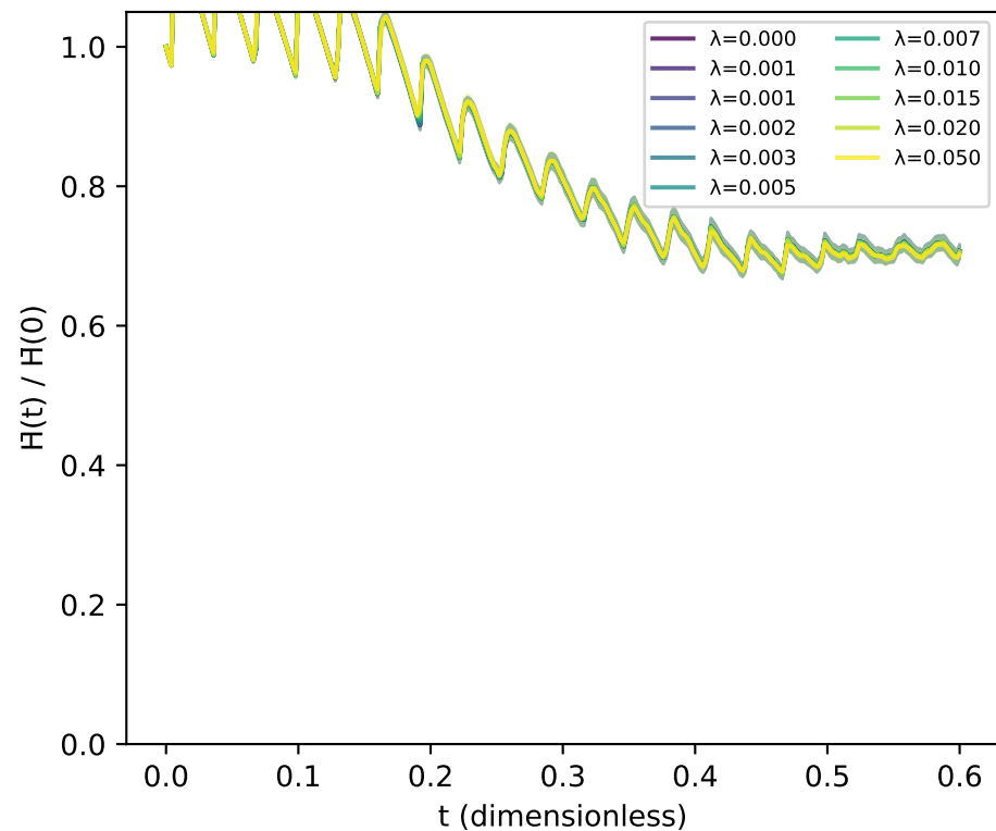
H-function evolution
