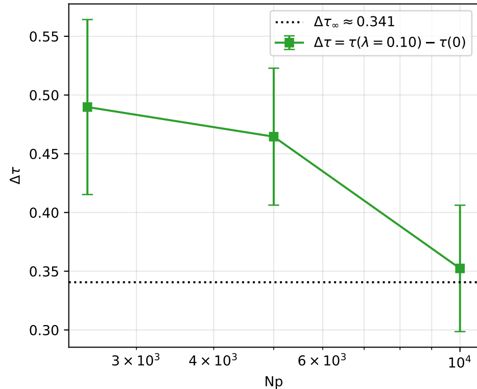
(c) Effect size vs N_p
