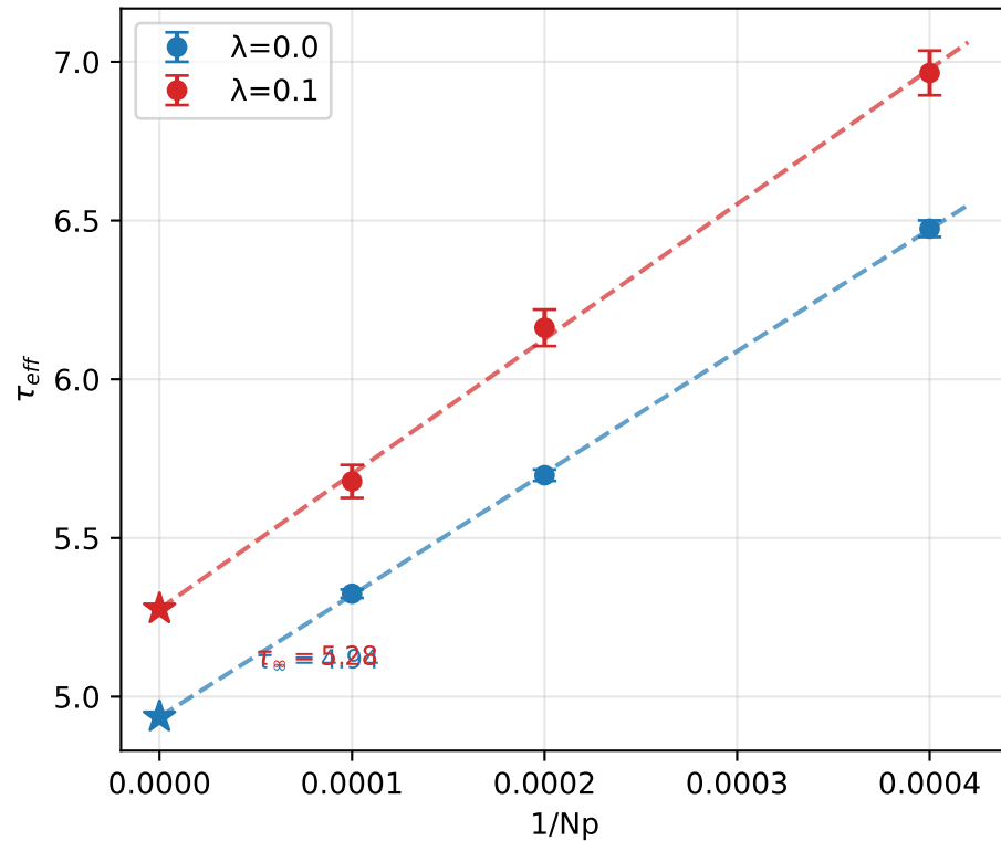
(b) \tau vs 1/N_p (linear fit \rightarrow \tau_\infty )
