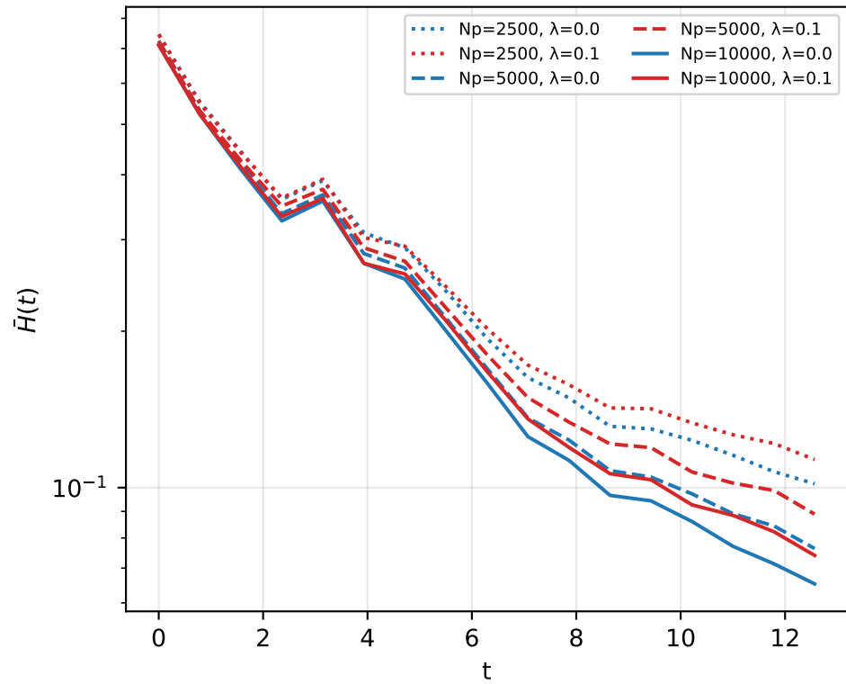
(a) \bar{H}(t) decay curves
