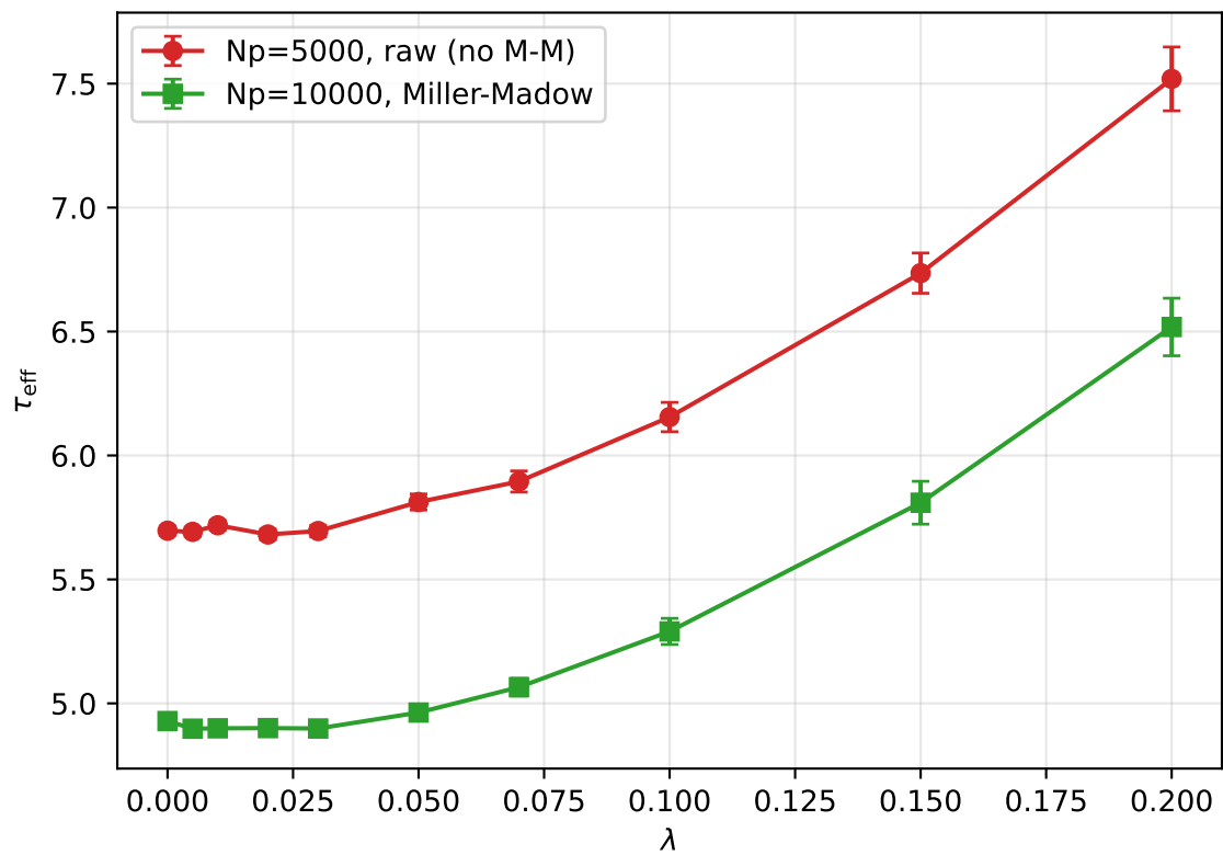
(a) \tau_{\text{eff}}(\lambda) : before/after audit
