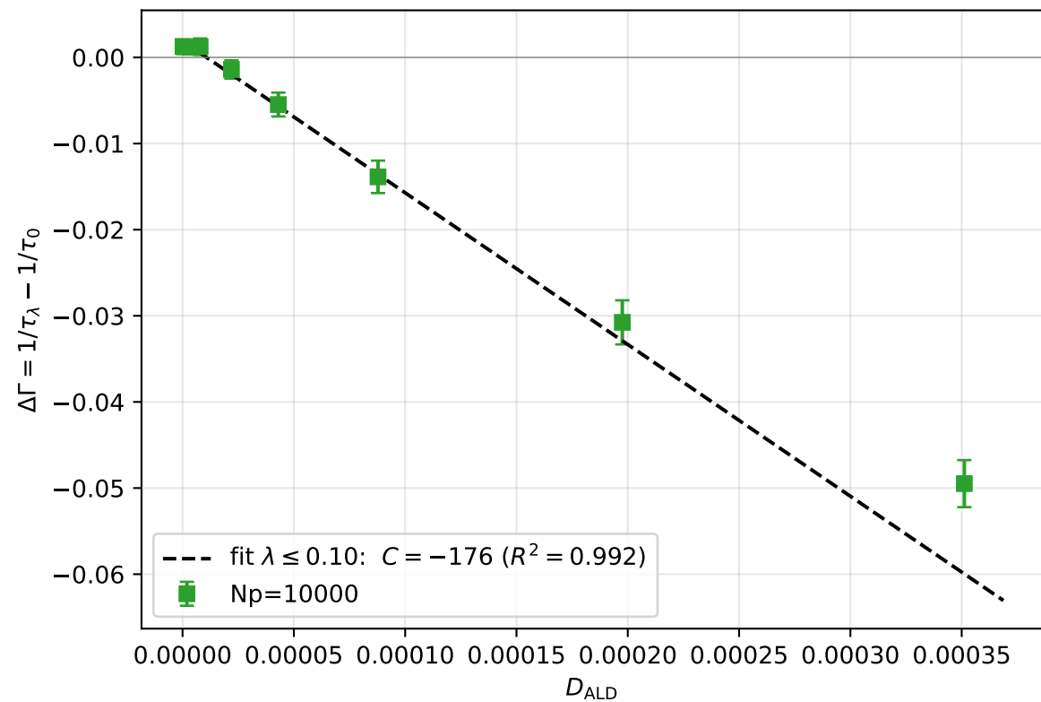
(b) \Delta\Gamma vs D_{\text{ALD}} - C < 0 : ZPF disrupts
