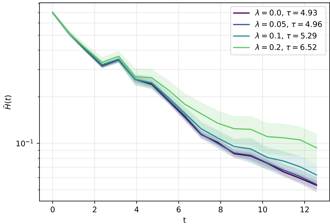
(c) H decay curves ( N_p=10000 , M-M corrected)
