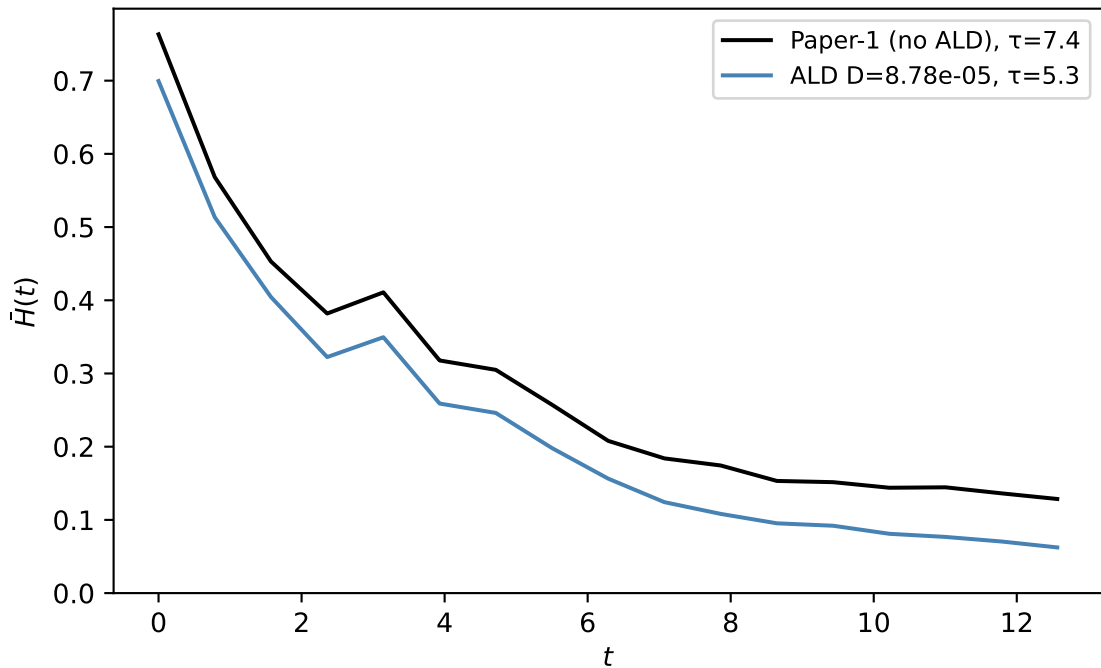
Born-rule relaxation: \lambda = 0.1
