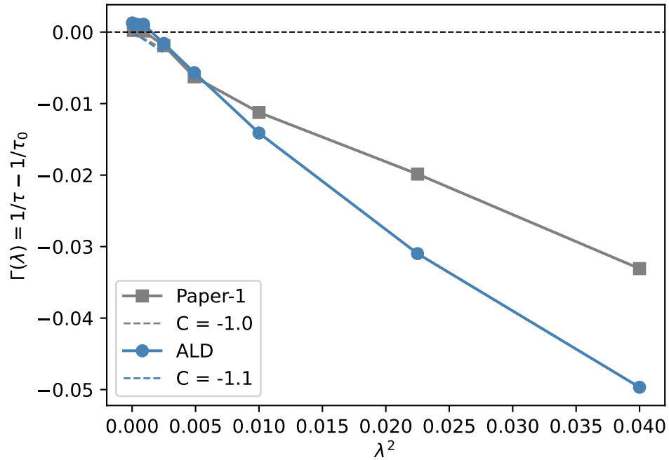
ZPF acceleration: \Gamma \propto C\lambda^2 ?
