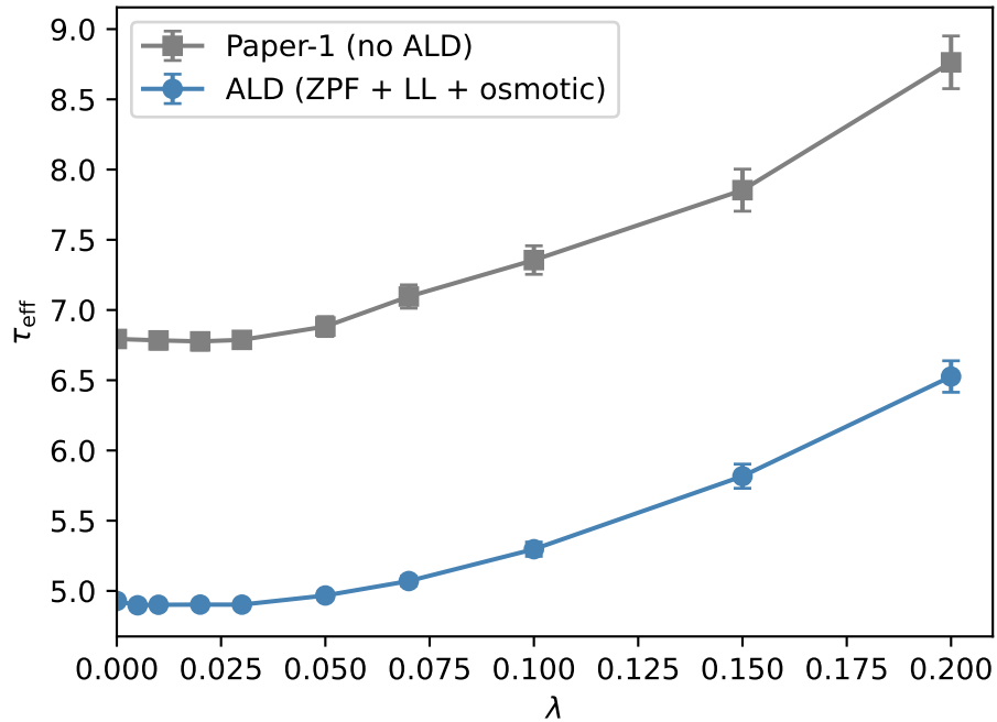
Relaxation time \tau_{\text{eff}}(\lambda)
