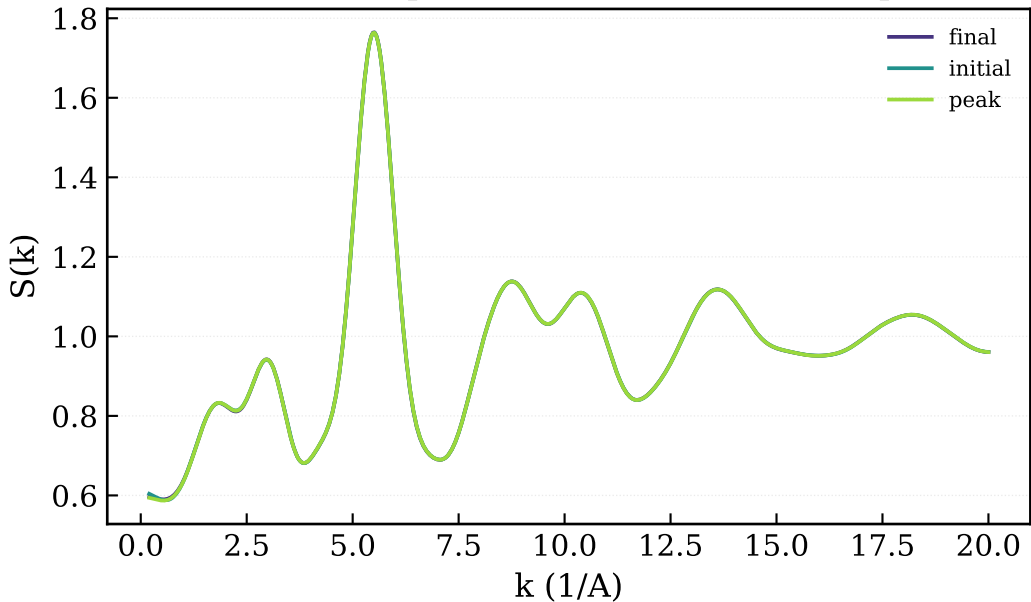
SK (initial/pico/final) - 25 keV / 20% sp3
