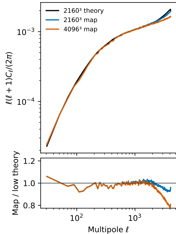
Summed map
