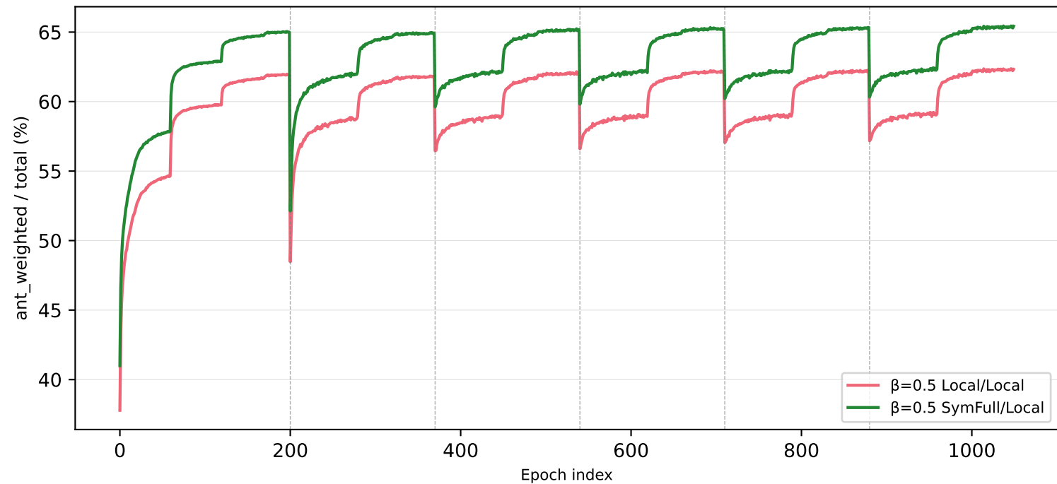
ANT weighted proportion of total loss — TIN 100-20
