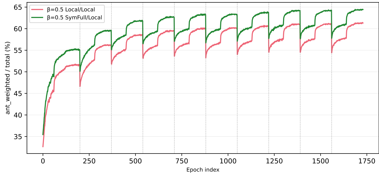
ANT weighted proportion of total loss — CIFAR-100 10-10
