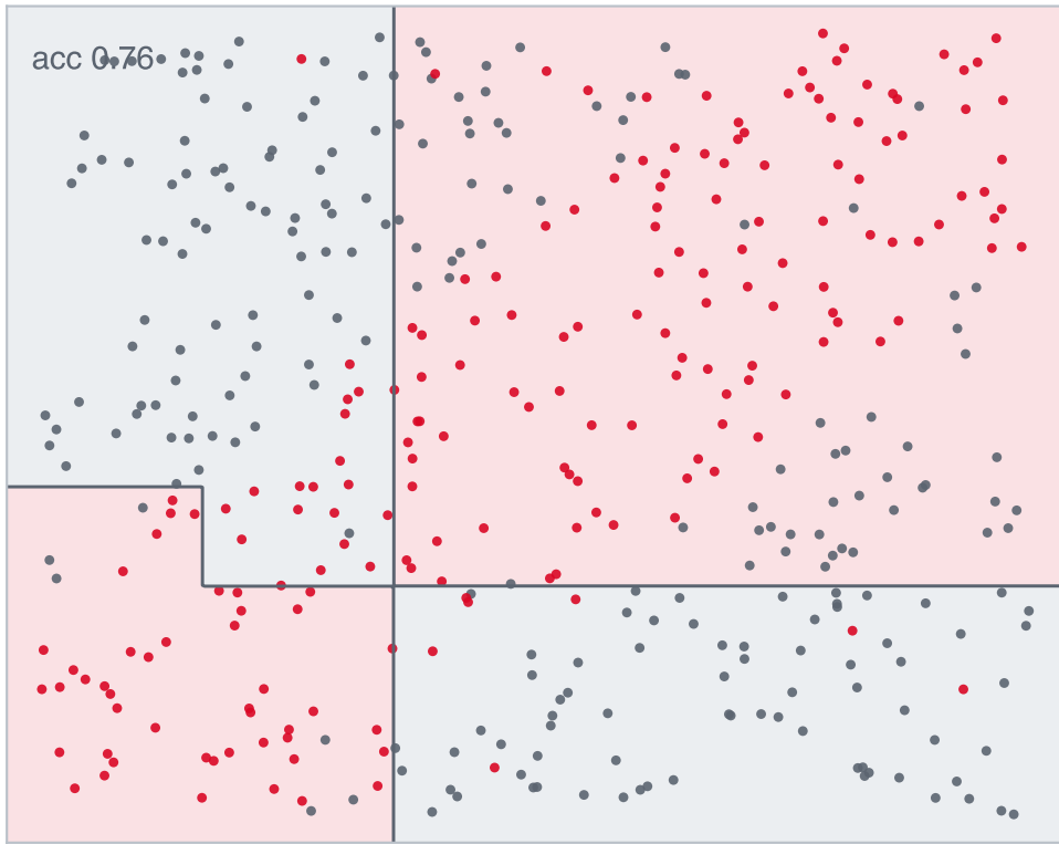
Axis-aligned tree (depth 3)
