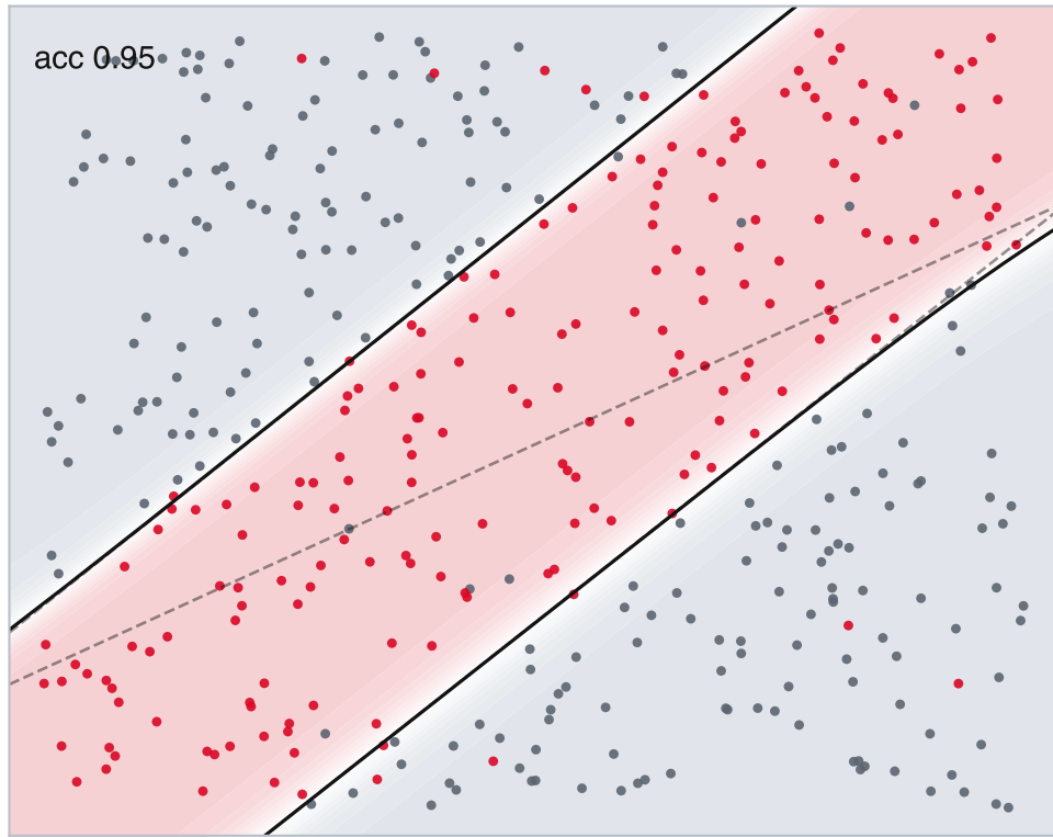
Soft-routed oblique tree (depth 2)
