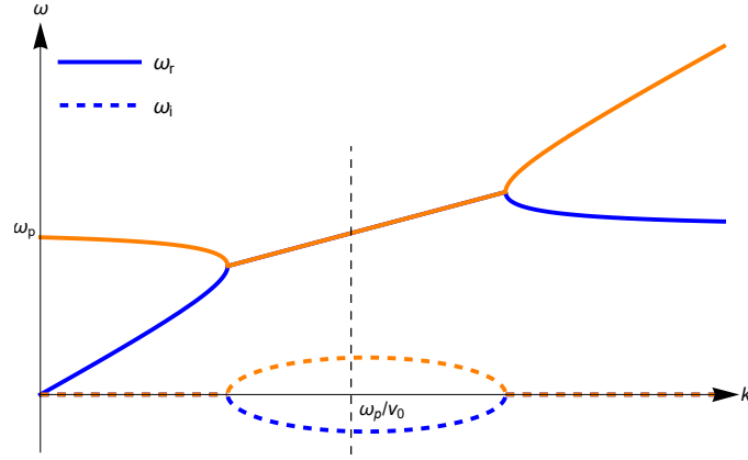
Figure 1.2: Sketch of \omega - k curves for the model dispersion relation of Eq. (1.4.7).
