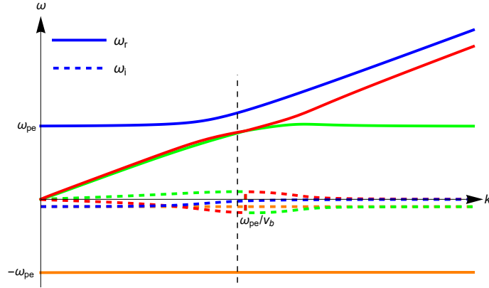
Figure 1.8: Negative-energy slow beam mode becomes unstable in the kv_b \gg \omega_{pe} limit due to positive collisional dissipation.
