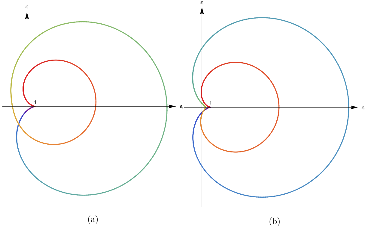
Figure 1.6: Nyquist diagram for the beam-plasma instability with (a) kv_b \ll \omega_{pe} and (b) kv_b \gg \omega_{pe} . The large semicircle C_R is mapped to \epsilon = 1 \pm i0 , and the image of the straight line C_\delta is colored with a rainbow gradient, where purple corresponds to \omega_r \rightarrow -\infty and red corresponds to \omega_r \rightarrow +\infty .
