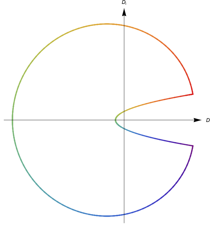
Figure 1.7: Nyquist diagram for the model ODE Eq. (1.5.10), which looks like the Pac-Man . The large semicircle C_R and the image of the straight line C_\delta are all colored with a rainbow gradient, where purple corresponds to \theta \rightarrow \pi or \omega_r \rightarrow -\infty and red corresponds to \theta \rightarrow 0 or \omega_r \rightarrow +\infty .
