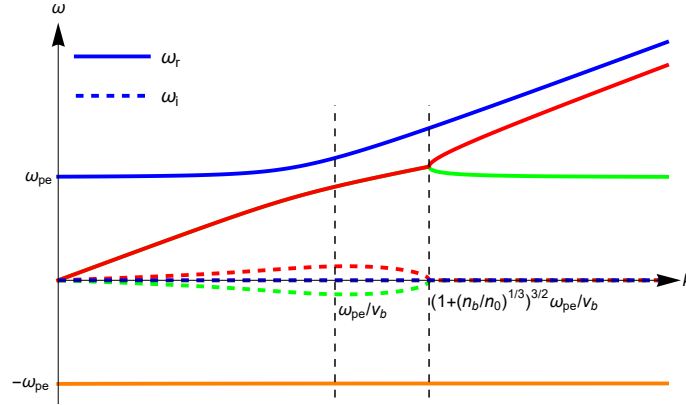
Figure 1.4: Sketch of \omega - k curves for the beam-plasma dispersion relation of Eq. (1.4.13).
