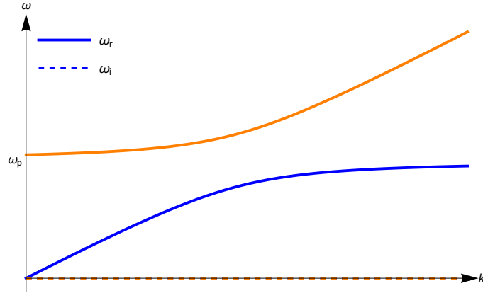
Figure 1.3: Sketch of \omega - k curves for the model dispersion relation of Eq. (1.4.12).
