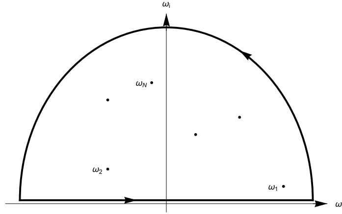
Figure 1.5: Integration contour in the complex \omega plane for Nyquist stability analysis.
