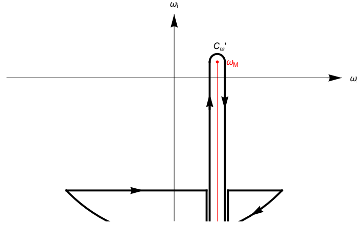
Figure 1.12: \omega integration contour which is consistent with the branch cut of \sqrt{\omega - \omega_M} .
