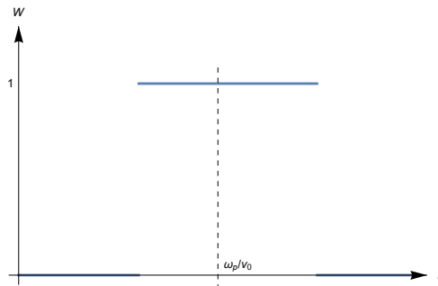
Figure 1.9: Winding number W as a function of k for the model dispersion relation Eq. (1.4.7) .
