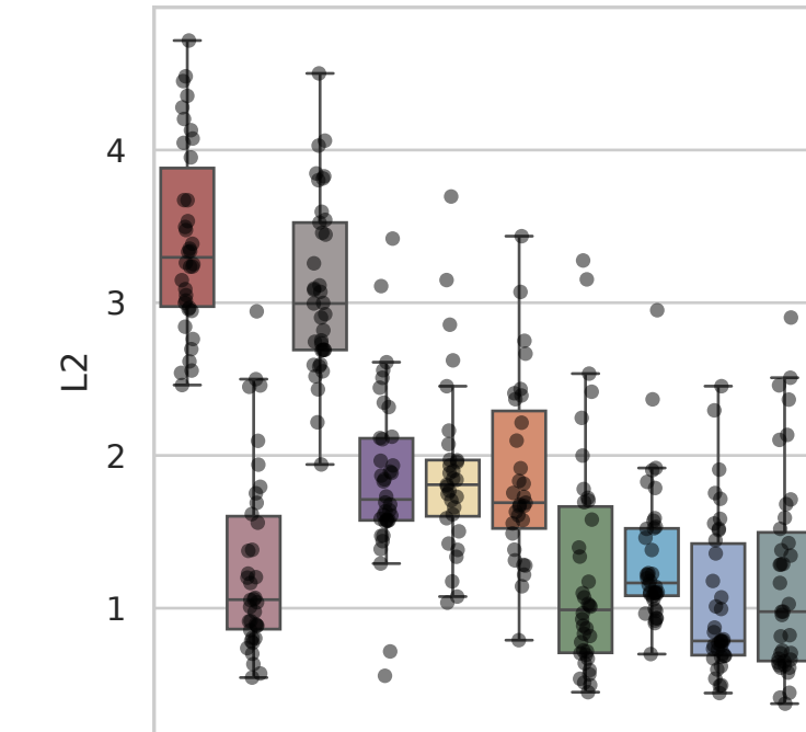
Dataset: Sunshine
