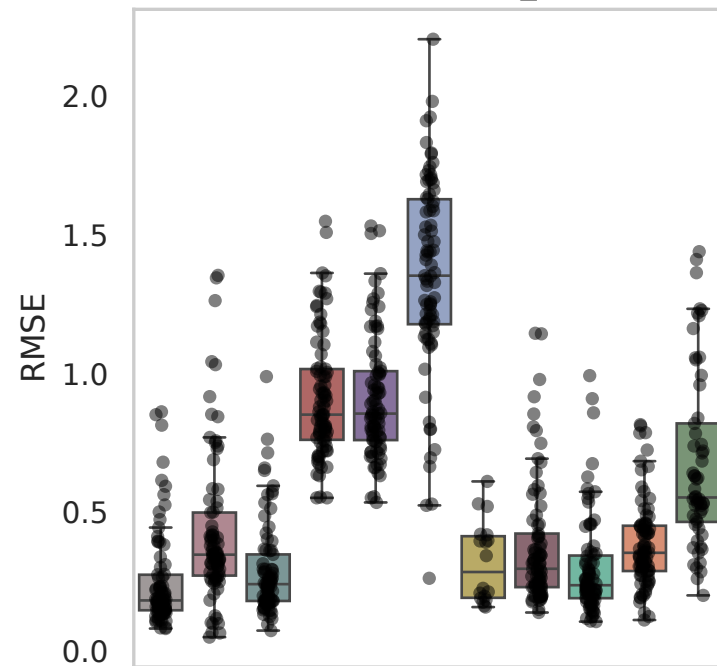
Dataset: Perturb_KHP
