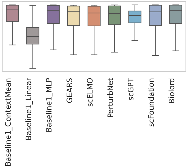
Pearson_Correlation_del Top20
