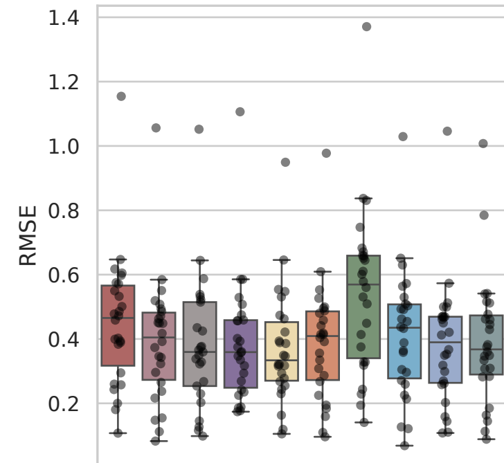
Dataset: Norman
