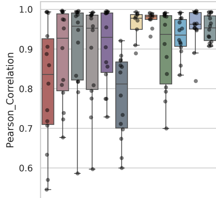
Dataset: Sunshine
