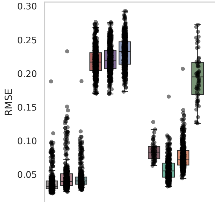
Dataset: Tahoe100
