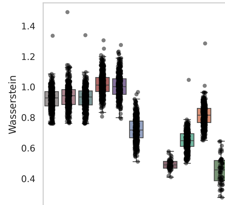
Dataset: Tahoe100
