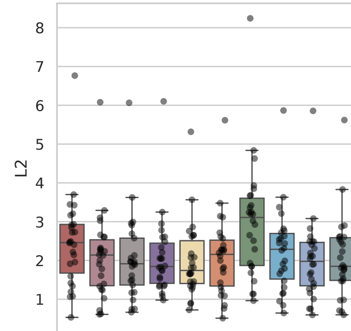
Dataset: Norman
