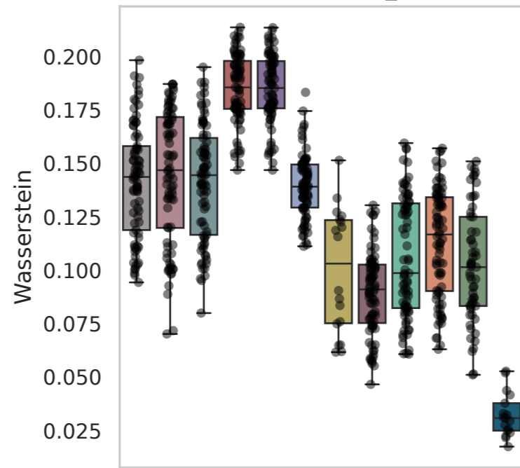
Dataset: Perturb_KHP
