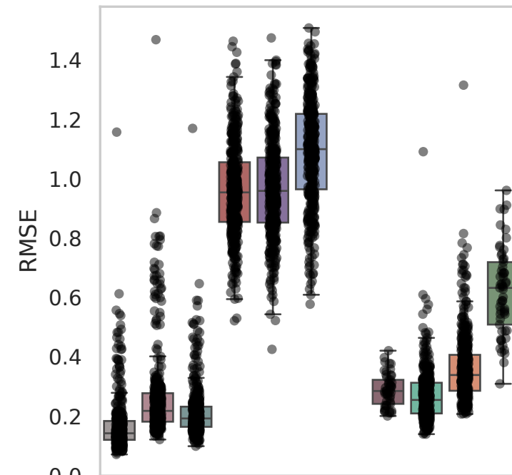
Dataset: Tahoe100
