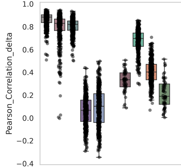
Dataset: Tahoe100
