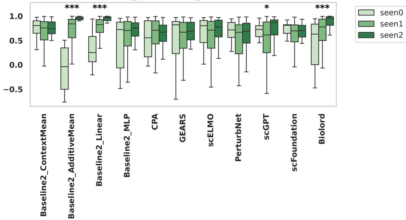
Pearson_Correlation_delta on Top20
