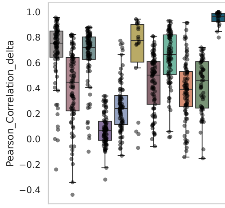
Dataset: Perturb_KHP
