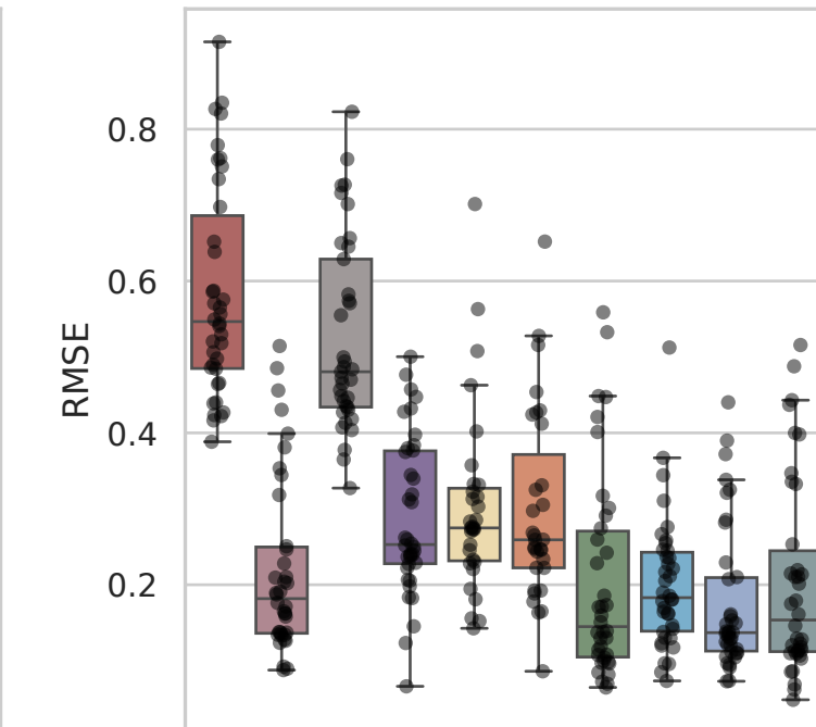
Dataset: Sunshine
