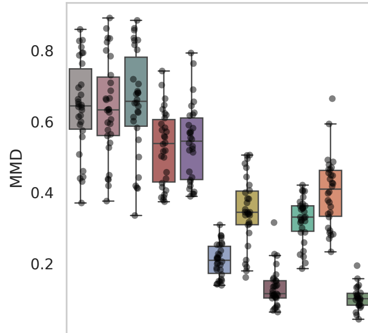
Dataset: Srivatsan
