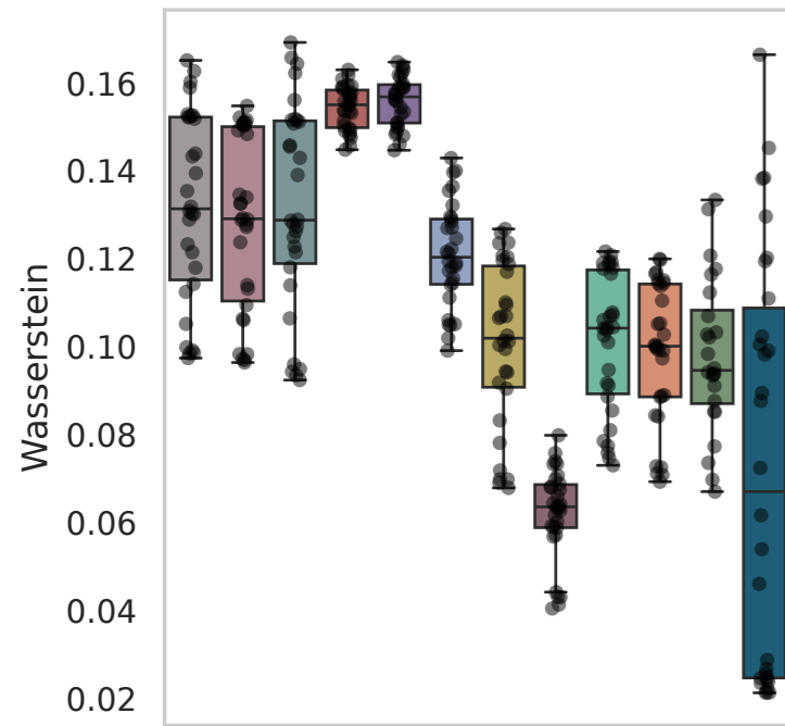
Dataset: Srivatsan
