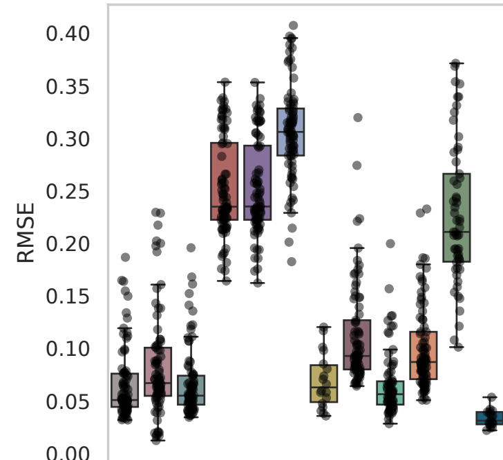
Dataset: Perturb_KHP
