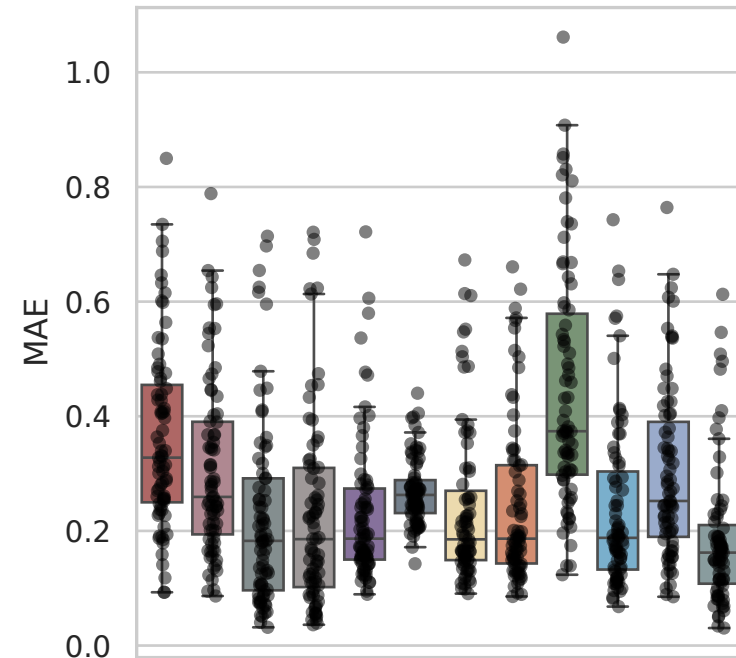
Dataset: Norman
