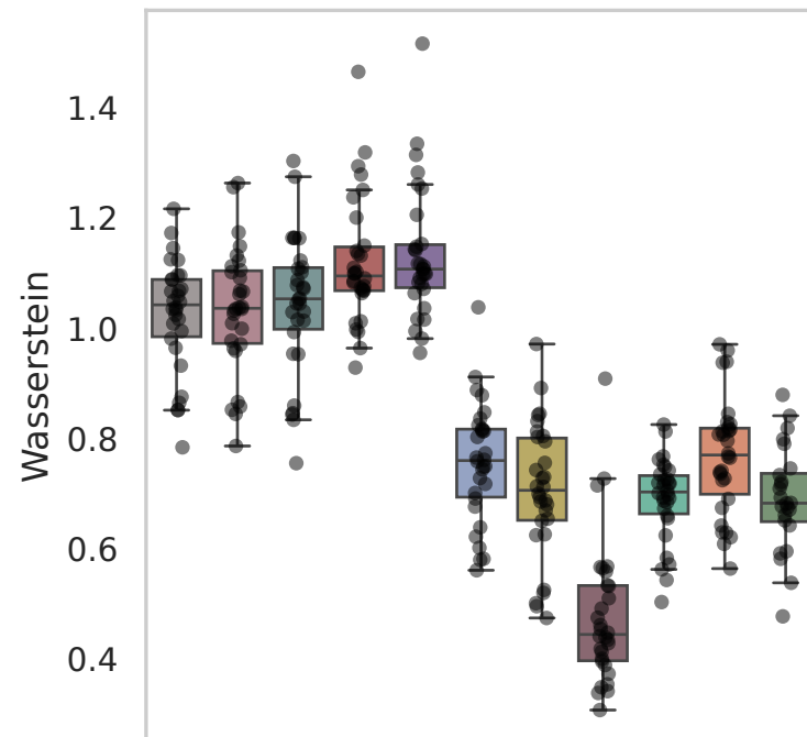
Dataset: Srivatsan
