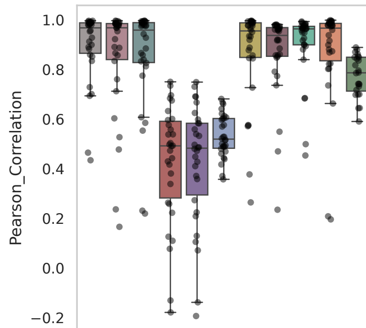
Dataset: Srivatsan
