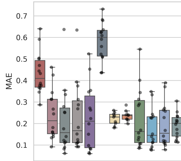
Dataset: Sunshine
