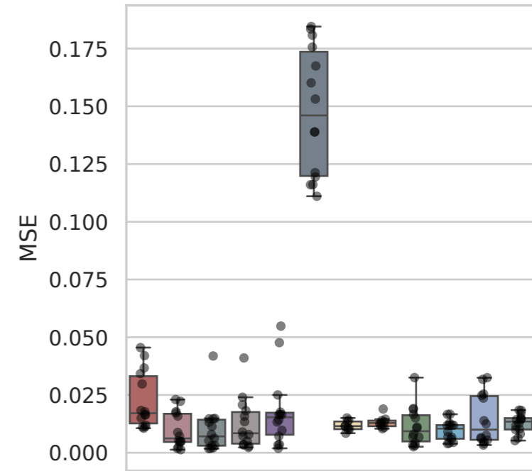
Dataset: Sunshine
