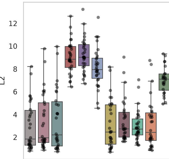
Dataset: Srivatsan
