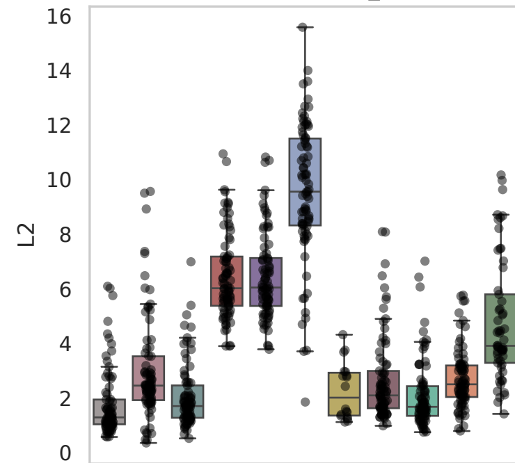
Dataset: Perturb_KHP
