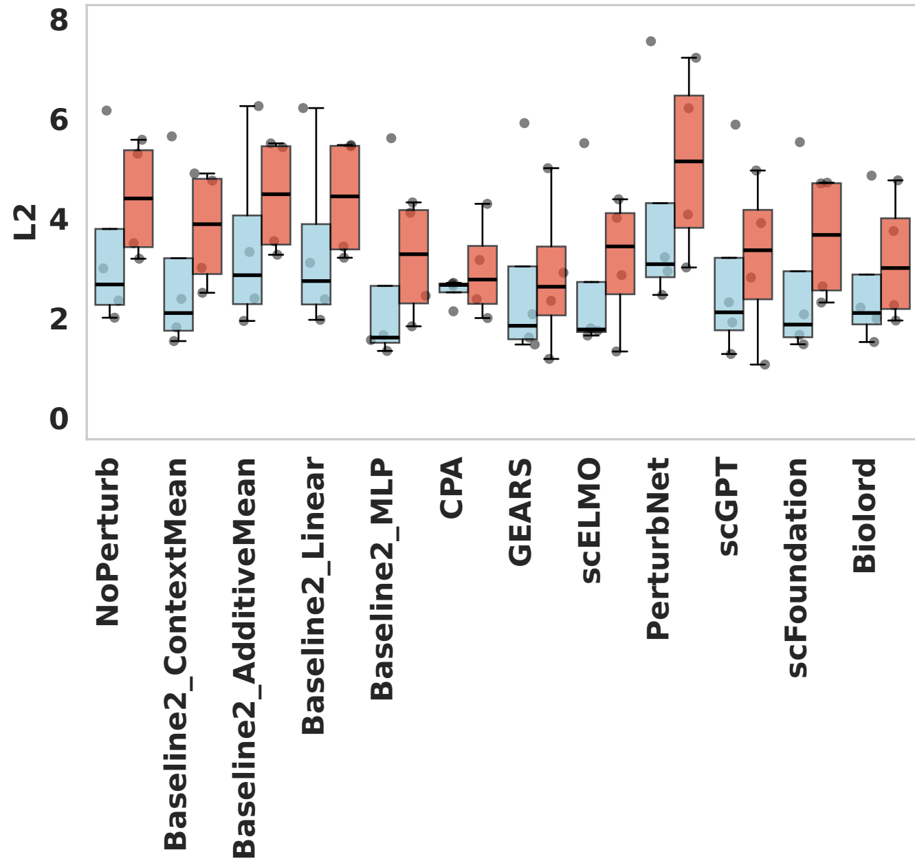
Seen0 Top50
