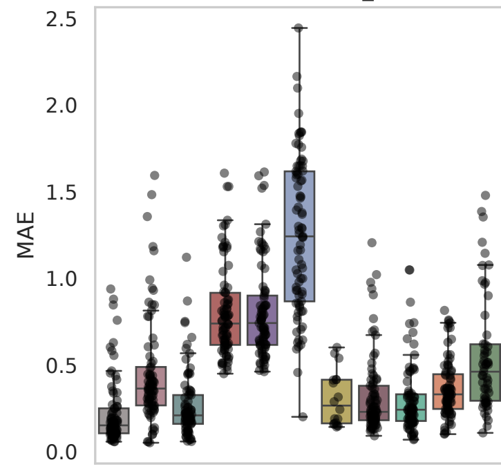
Dataset: Perturb_KHP
