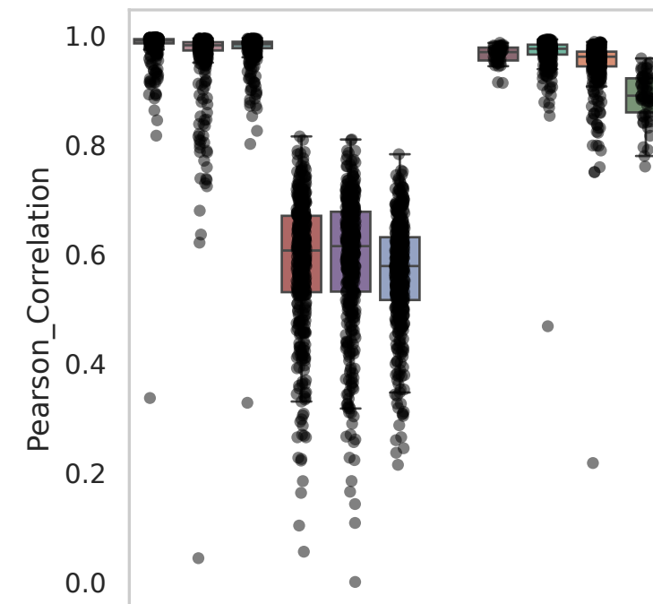
Dataset: Tahoe100
