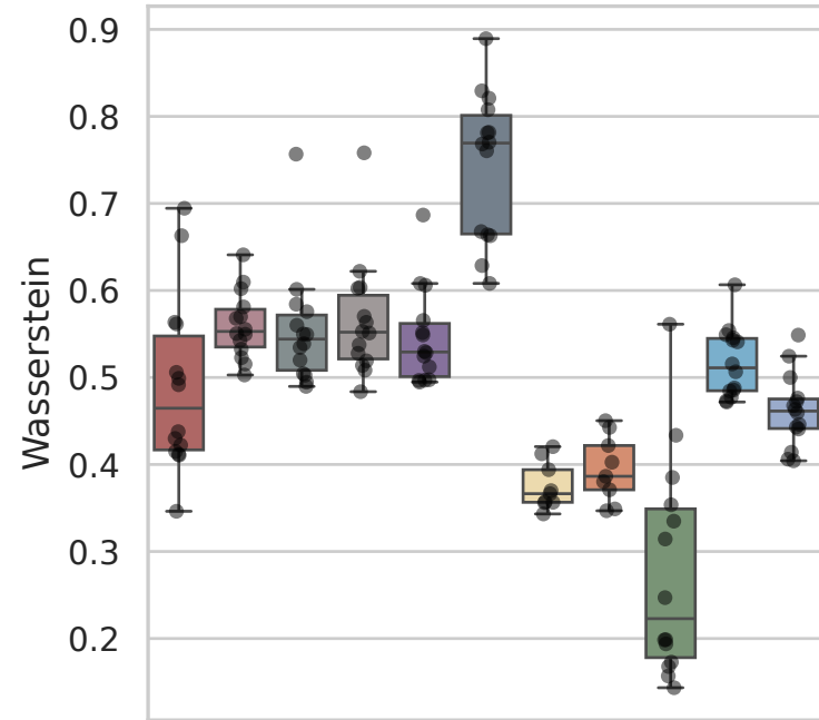
Dataset: Sunshine
