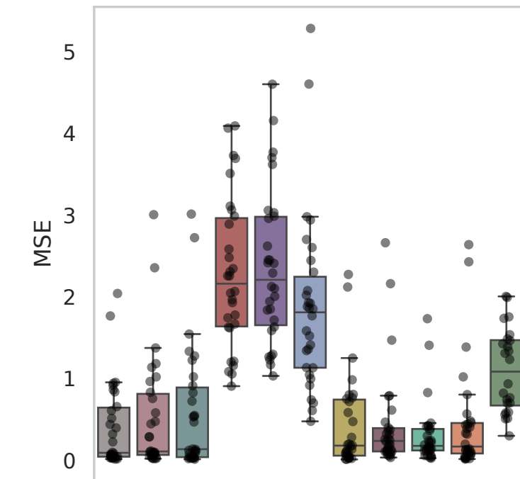
Dataset: Srivatsan
