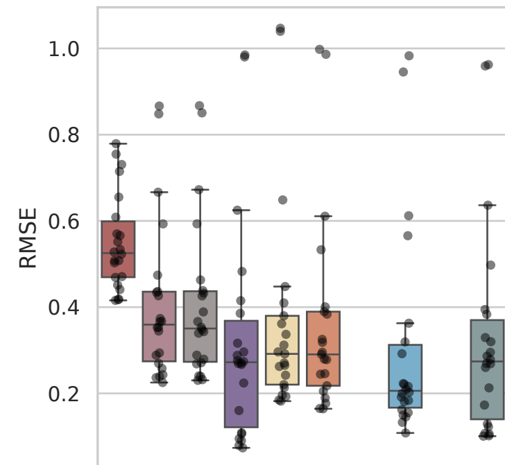
Dataset: Adamson
