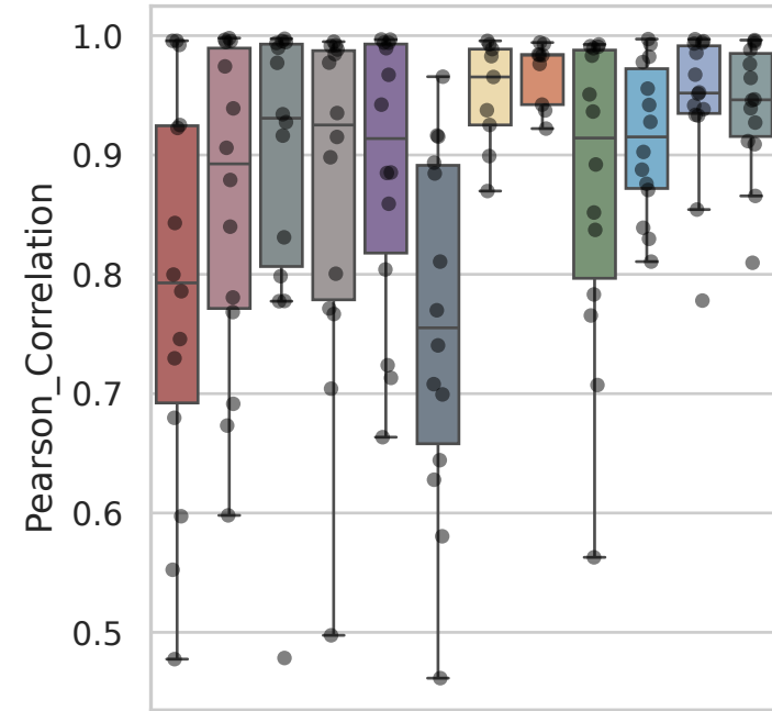
Dataset: Sunshine
