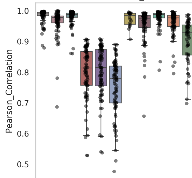
Dataset: Perturb_KHP
