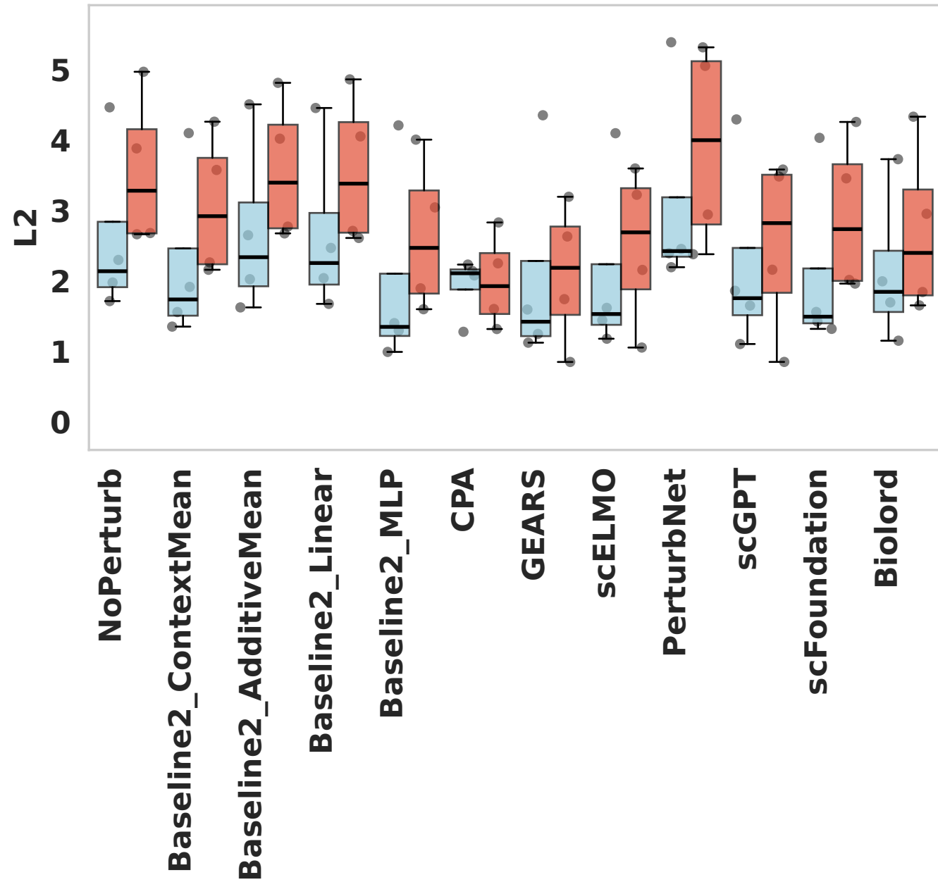
Seen0 Top20
