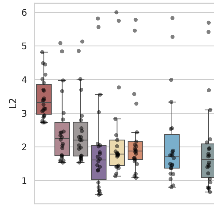
Dataset: Adamson
