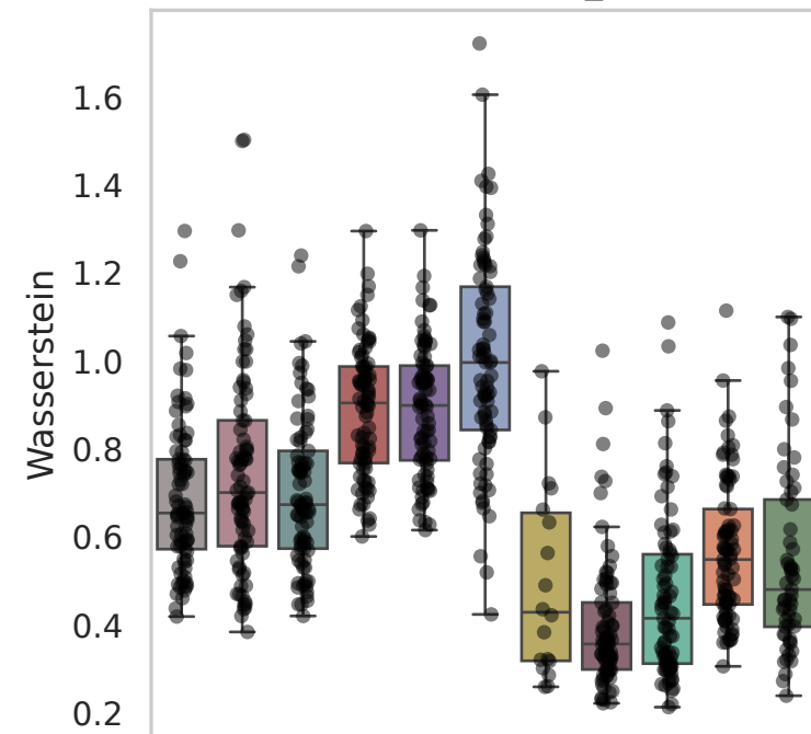
Dataset: Perturb_KHP
