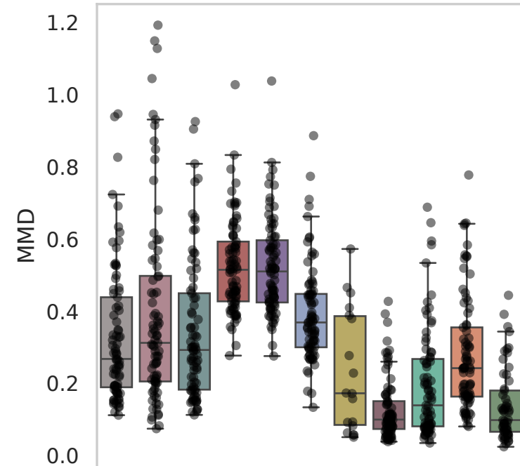
Dataset: Perturb_KHP
