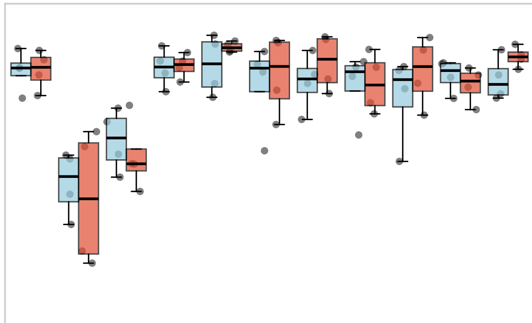
Seen0 Top100
