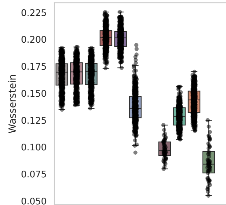
Dataset: Tahoe100
