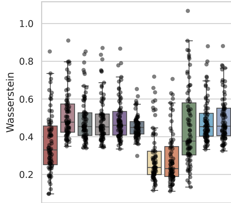
Dataset: Norman
