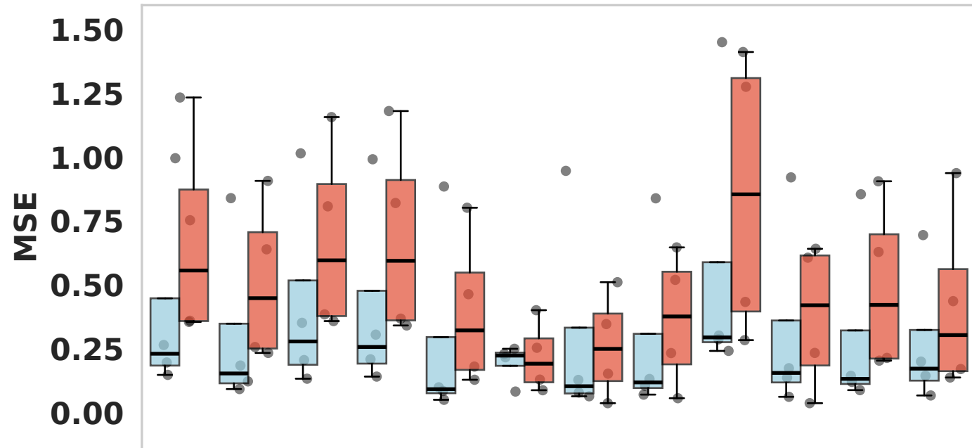
Seen0 Top20
