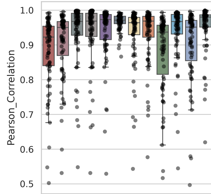
Dataset: Norman
