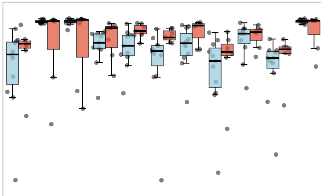
Seen2 Top100
