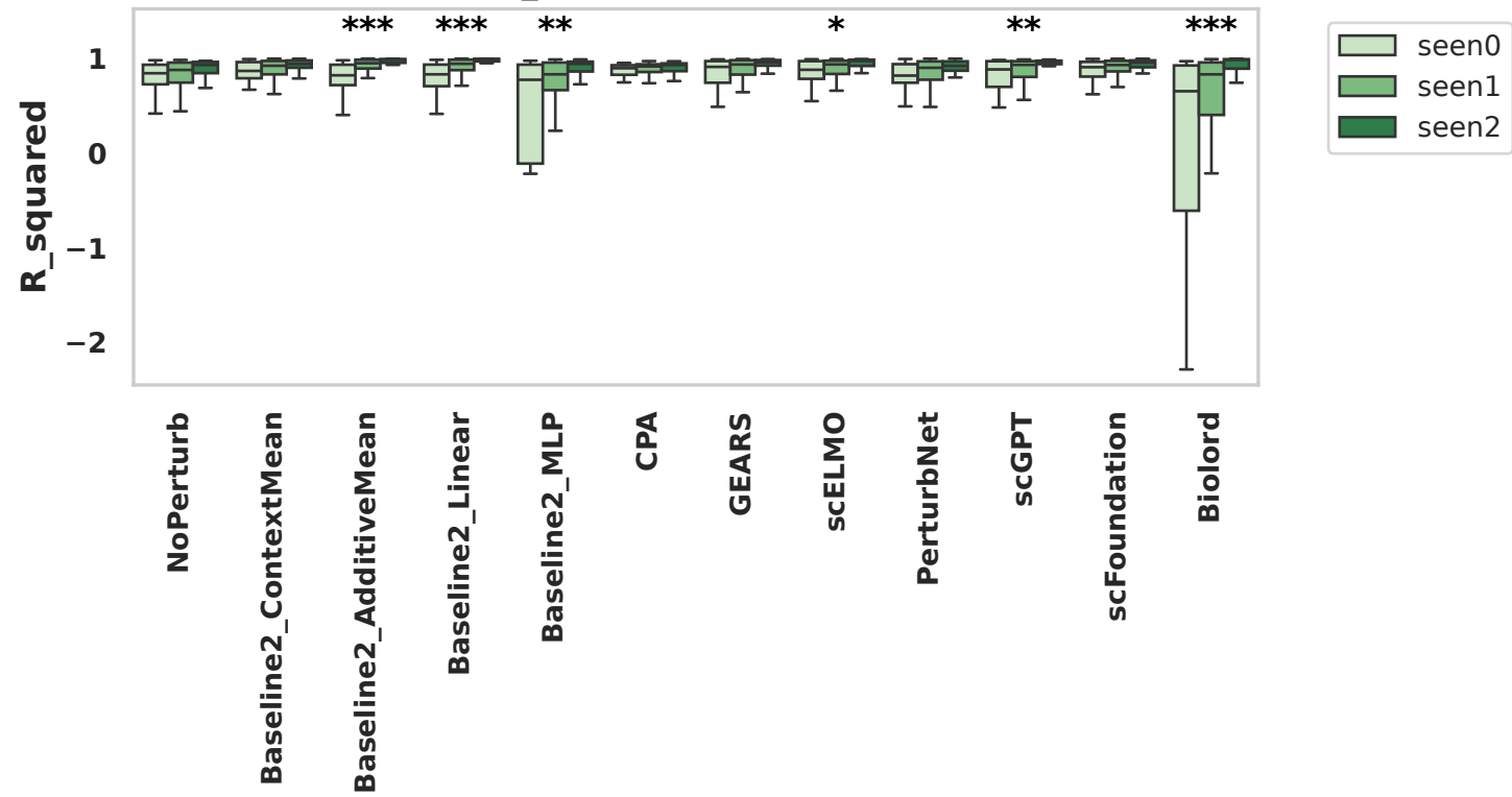
R_squared on Top100
