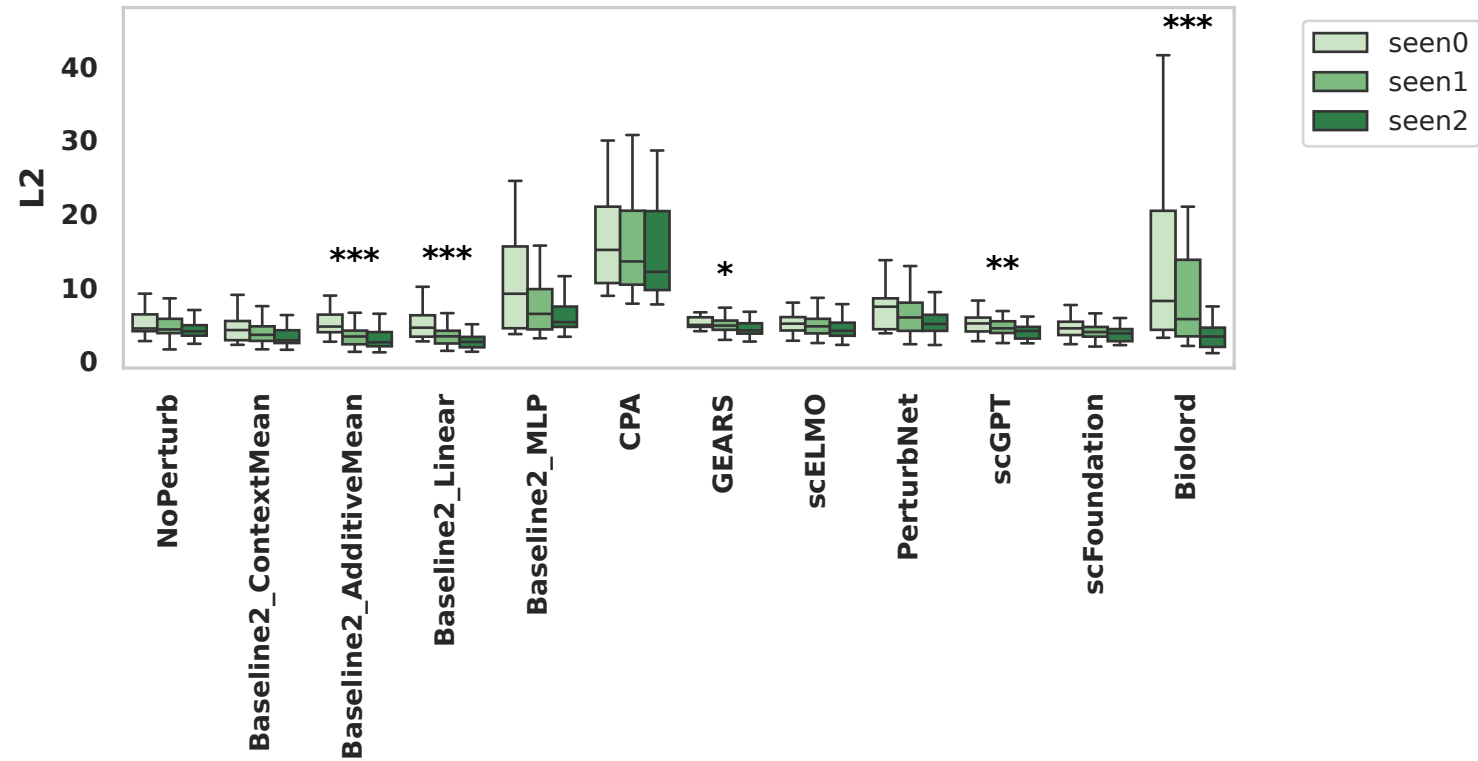
L2 on Allgenes
