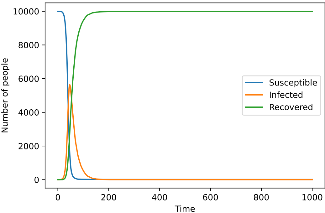
SIR Model Simulation
